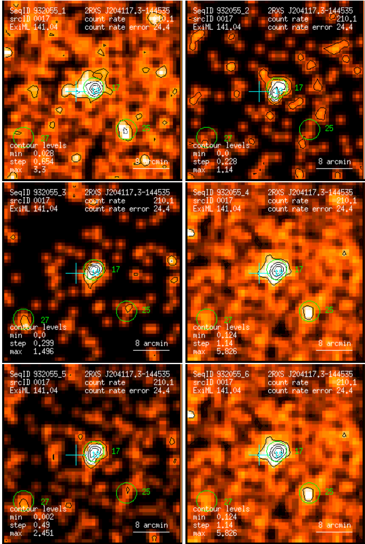
Figure 17: RASS 932055: detection 0017: band rate images, Gaussian filter: (1) PSPC channels 11 – 41, (2) 52 – 90, (3) 91 – 201, (4) 11 – 235, (5) 52 – 201, (6) 11 – 201. Broad band rates in counts/ks. Band rate contour levels in counts/ks/arcmin 2 .
