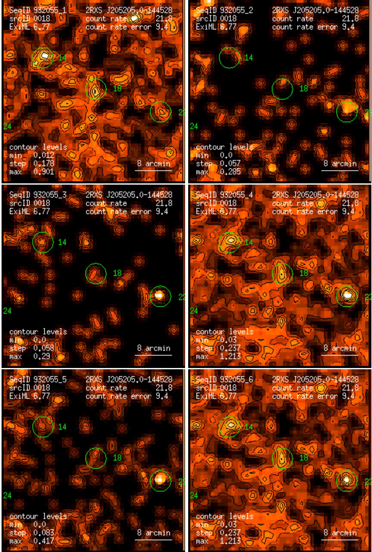
Figure 18: RASS 932055: detection 0018: band rate images, Gaussian filter: (1) PSPC channels 11 – 41, (2) 52 – 90, (3) 91 – 201, (4) 11 – 235, (5) 52 – 201, (6) 11 – 201. Broad band rates in counts/ks. Band rate contour levels in counts/ks/arcmin 2 .
