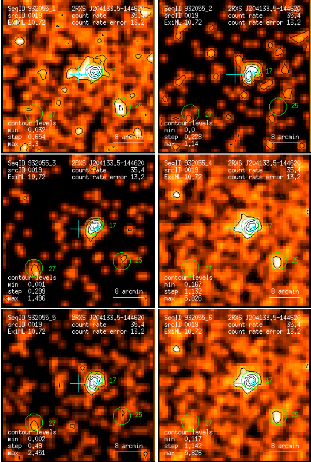
Figure 19: RASS 932055: detection 0019: band rate images, Gaussian filter: (1) PSPC channels 11 – 41, (2) 52 – 90, (3) 91 – 201, (4) 11 – 235, (5) 52 – 201, (6) 11 – 201. Broad band rates in counts/ks. Band rate contour levels in counts/ks/arcmin 2 .
