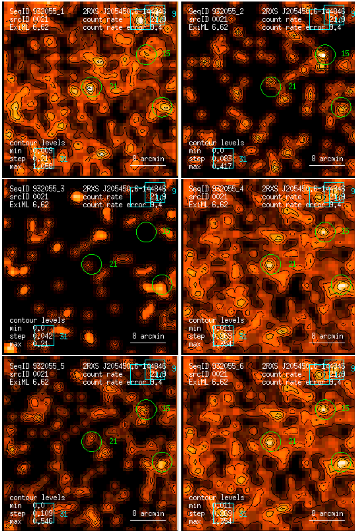
Figure 21: RASS 932055: detection 0021: band rate images, Gaussian filter: (1) PSPC channels 11 – 41, (2) 52 – 90, (3) 91 – 201, (4) 11 – 235, (5) 52 – 201, (6) 11 – 201. Broad band rates in counts/ks. Band rate contour levels in counts/ks/arcmin 2 .
