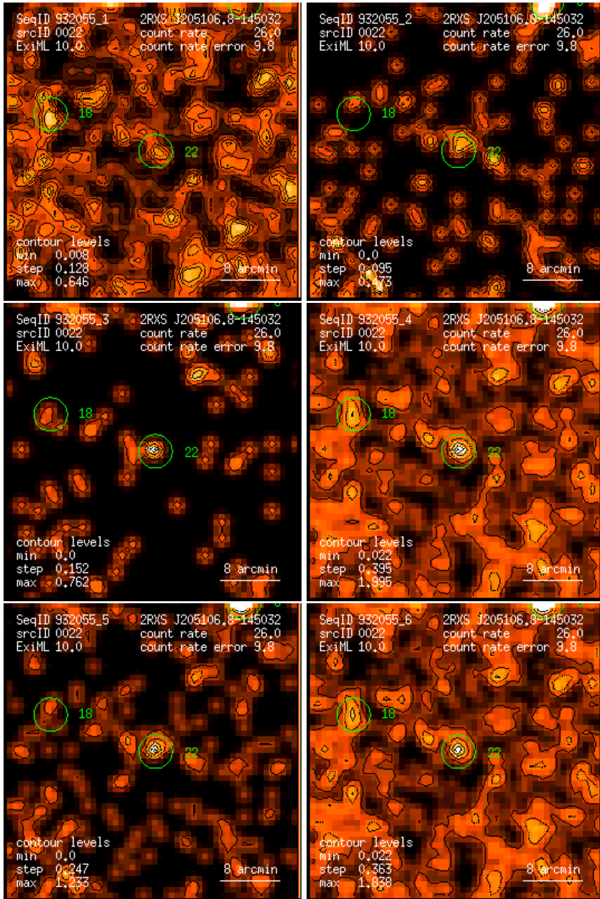
Figure 22: RASS 932055: detection 0022: band rate images, Gaussian filter: (1) PSPC channels 11 – 41, (2) 52 – 90, (3) 91 – 201, (4) 11 – 235, (5) 52 – 201, (6) 11 – 201. Broad band rates in counts/ks. Band rate contour levels in counts/ks/arcmin 2 .
