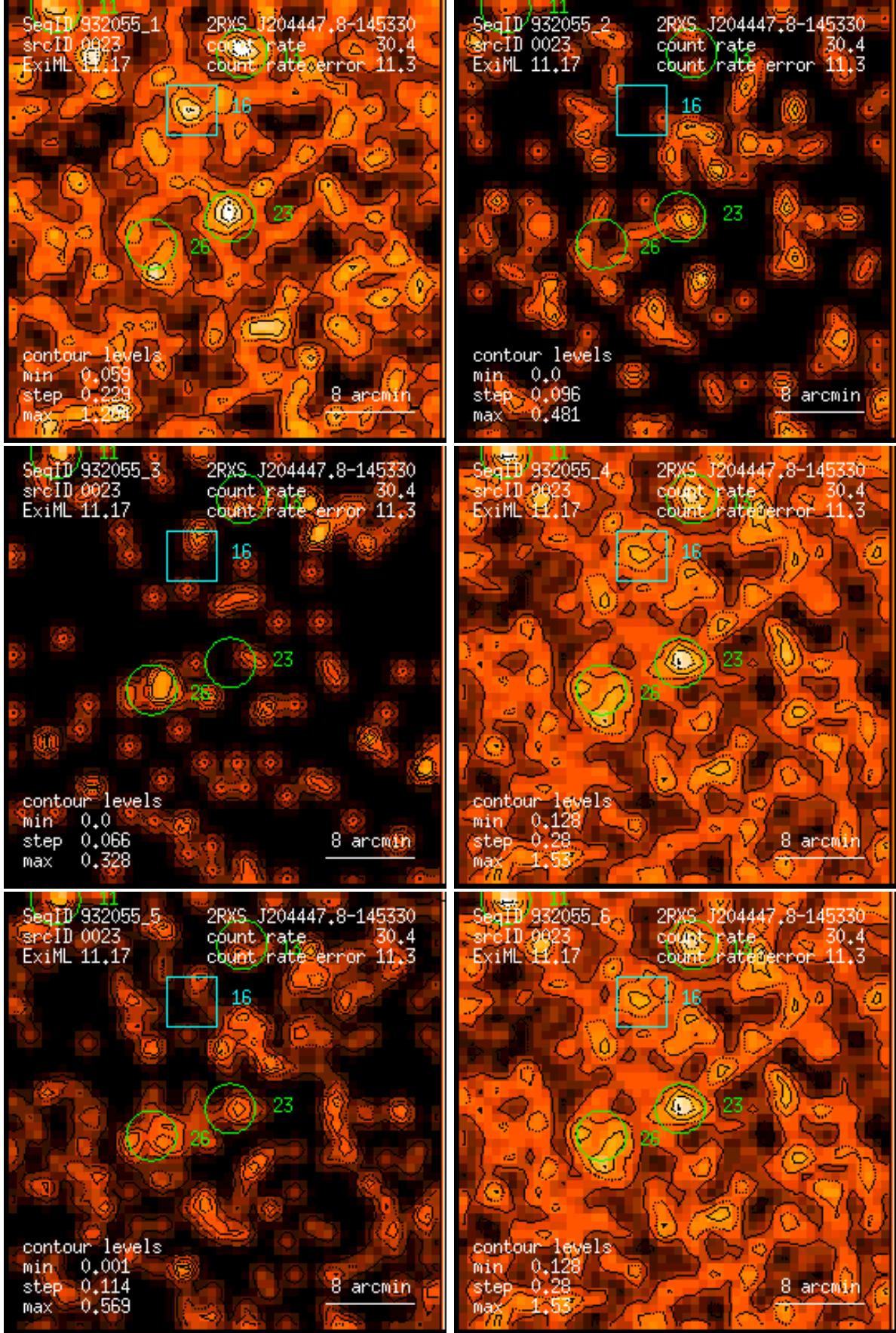
Figure 23: RASS 932055: detection 0023: band rate images, Gaussian filter: (1) PSPPC channels 11 – 41, (2) 52 – 90, (3) 91 – 201, (4) 11 – 235, (5) 52 – 201, (6) 11 – 201. Broad band rates in counts/ks. Band rate contour levels in counts/ks/arcmin 2 .
