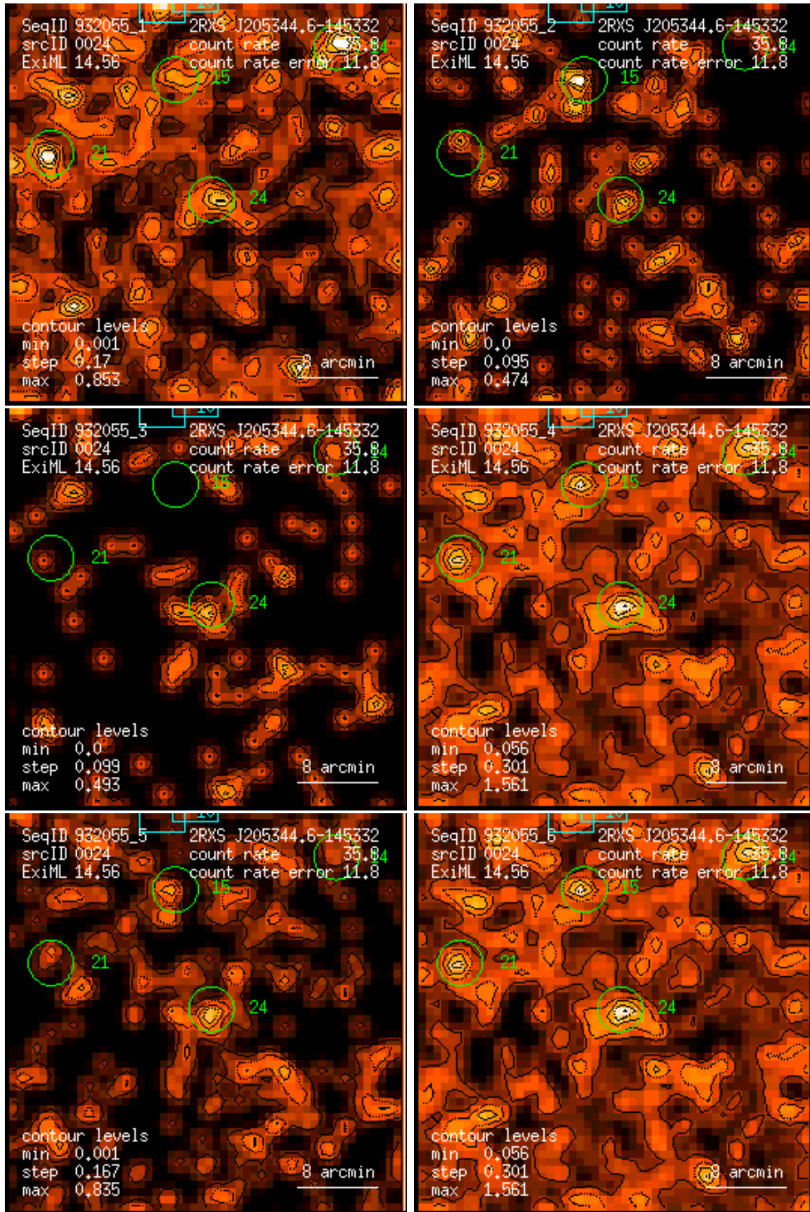
Figure 24: RASS 932055: detection 0024: band rate images, Gaussian filter: (1) PSPC channels 11 – 41, (2) 52 – 90, (3) 91 – 201, (4) 11 – 235, (5) 52 – 201, (6) 11 – 201. Broad band rates in counts/ks. Band rate contour levels in counts/ks/arcmin 2 .
