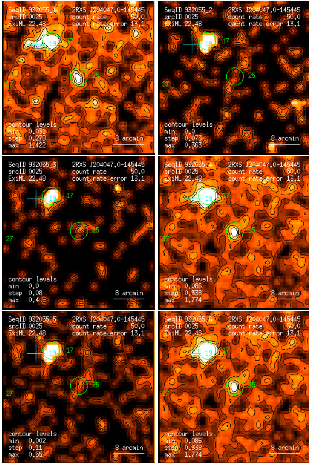
Figure 25: RASS 932055: detection 0025: band rate images, Gaussian filter: (1) PSPC channels 11 – 41, (2) 52 – 90, (3) 91 – 201, (4) 11 – 235, (5) 52 – 201, (6) 11 – 201. Broad band rates in counts/ks. Band rate contour levels in counts/ks/arcmin 2 .
