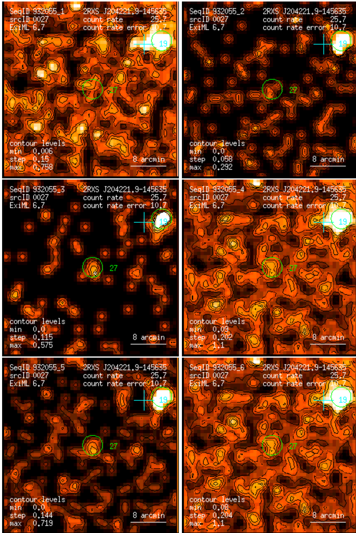
Figure 27: RASS 932055: detection 0027: band rate images, Gaussian filter: (1) PSPC channels 11 – 41, (2) 52 – 90, (3) 91 – 201, (4) 11 – 235, (5) 52 – 201, (6) 11 – 201. Broad band rates in counts/ks. Band rate contour levels in counts/ks/arcmin 2 .
