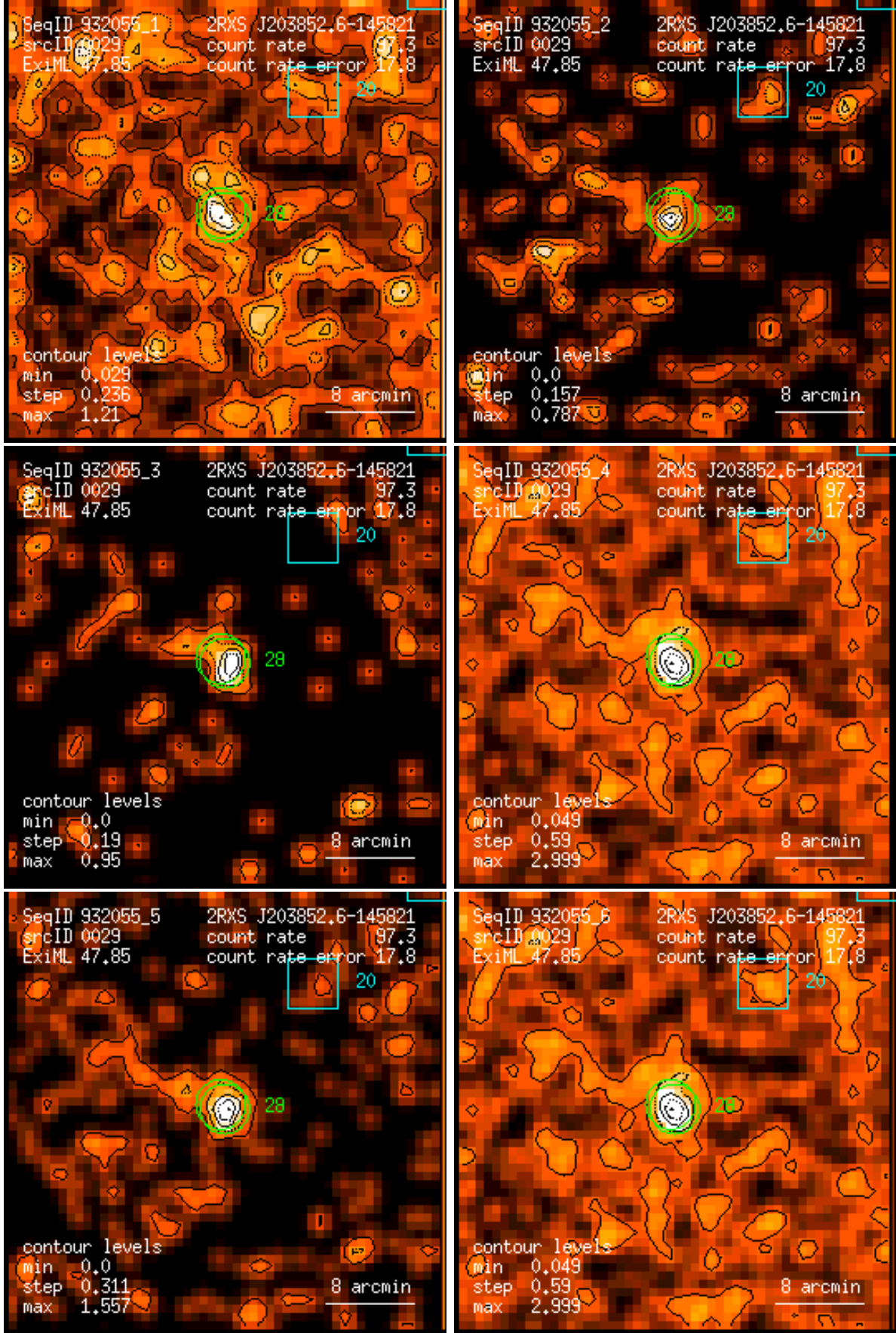
Figure 29: RASS 932055: detection 0029: band rate images, Gaussian filter: (1) PSPC channels 11 – 41, (2) 52 – 90, (3) 91 – 201, (4) 11 – 235, (5) 52 – 201, (6) 11 – 201. Broad band rates in counts/ks. Band rate contour levels in counts/ks/arcmin 2 .
