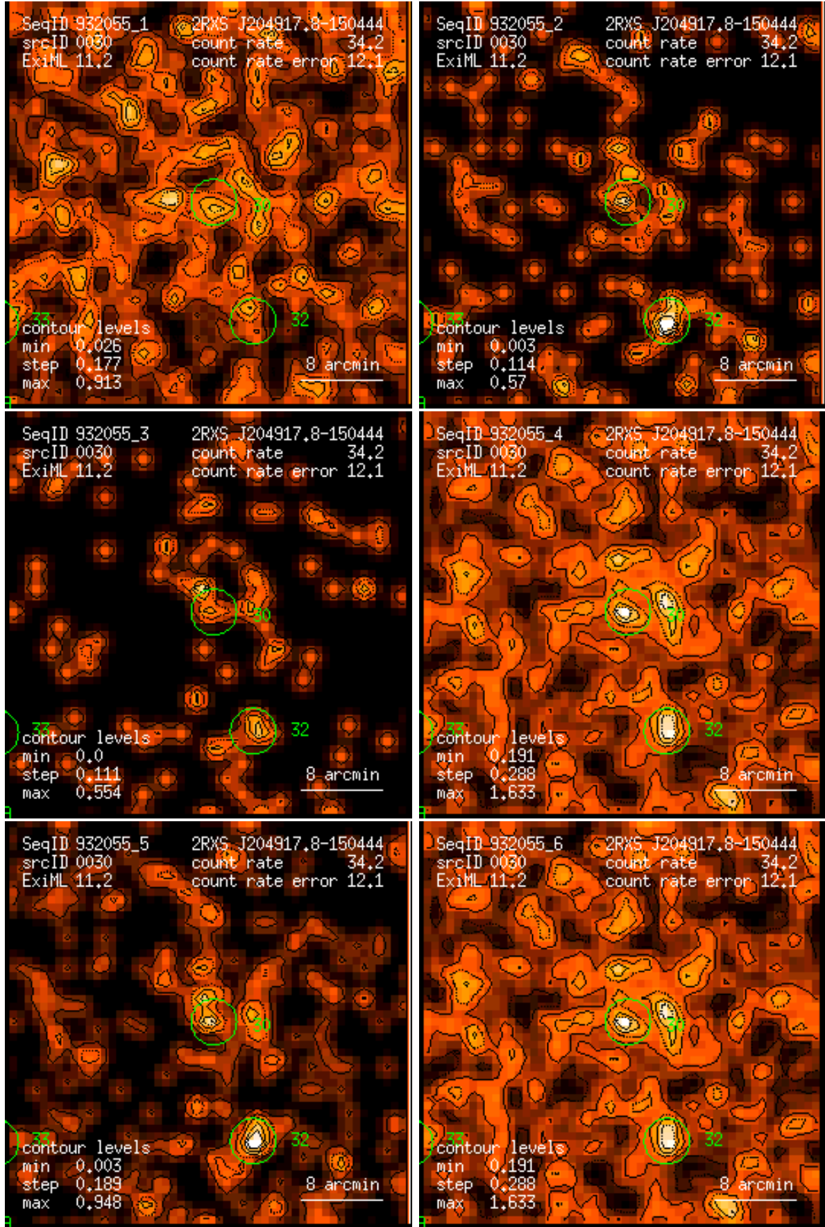
Figure 30: RASS 932055: detection 0030: band rate images, Gaussian filter: (1) PSPC channels 11 – 41, (2) 52 – 90, (3) 91 – 201, (4) 11 – 235, (5) 52 – 201, (6) 11 – 201. Broad band rates in counts/ks. Band rate contour levels in counts/ks/arcmin 2 .
