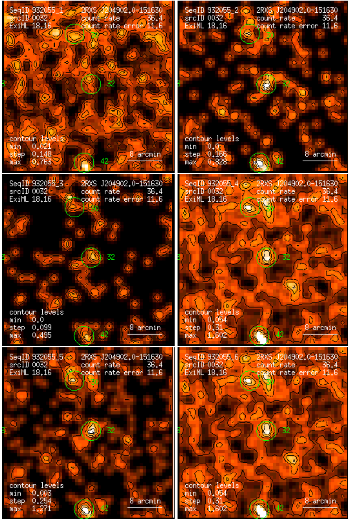
Figure 32: RASS 932055: detection 0032: band rate images, Gaussian filter: (1) PSPC channels 11 – 41, (2) 52 – 90, (3) 91 – 201, (4) 11 – 235, (5) 52 – 201, (6) 11 – 201. Broad band rates in counts/ks. Band rate contour levels in counts/ks/arcmin 2 .
