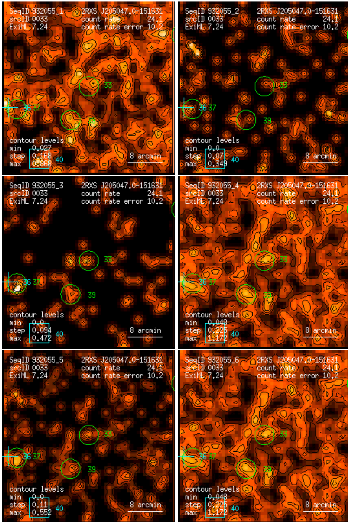
Figure 33: RASS 932055: detection 0033: band rate images, Gaussian filter: (1) PSPC channels 11 – 41, (2) 52 – 90, (3) 91 – 201, (4) 11 – 235, (5) 52 – 201, (6) 11 – 201. Broad band rates in counts/ks. Band rate contour levels in counts/ks/arcmin 2 .
