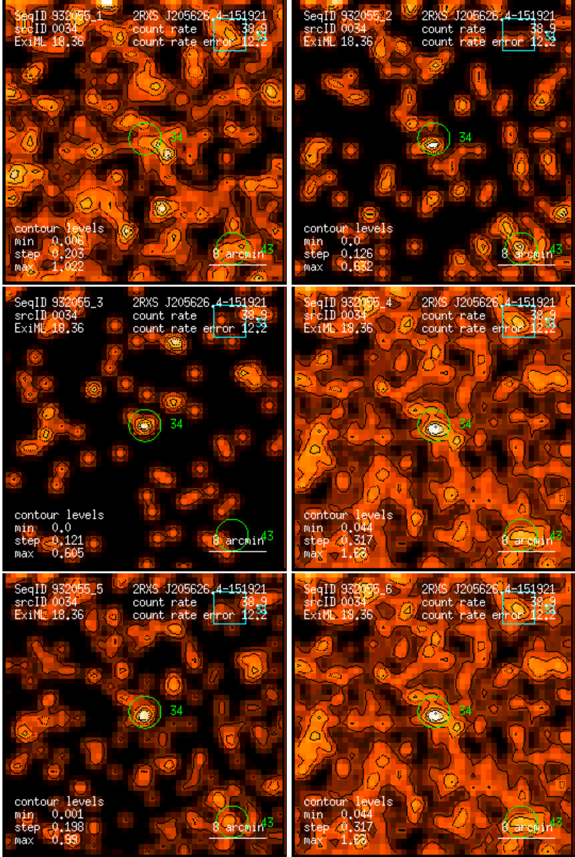
Figure 34: RASS 932055: detection 0034: band rate images, Gaussian filter: (1) PSPC channels 11 – 41, (2) 52 – 90, (3) 91 – 201, (4) 11 – 235, (5) 52 – 201, (6) 11 – 201. Broad band rates in counts/ks. Band rate contour levels in counts/ks/arcmin 2 .
