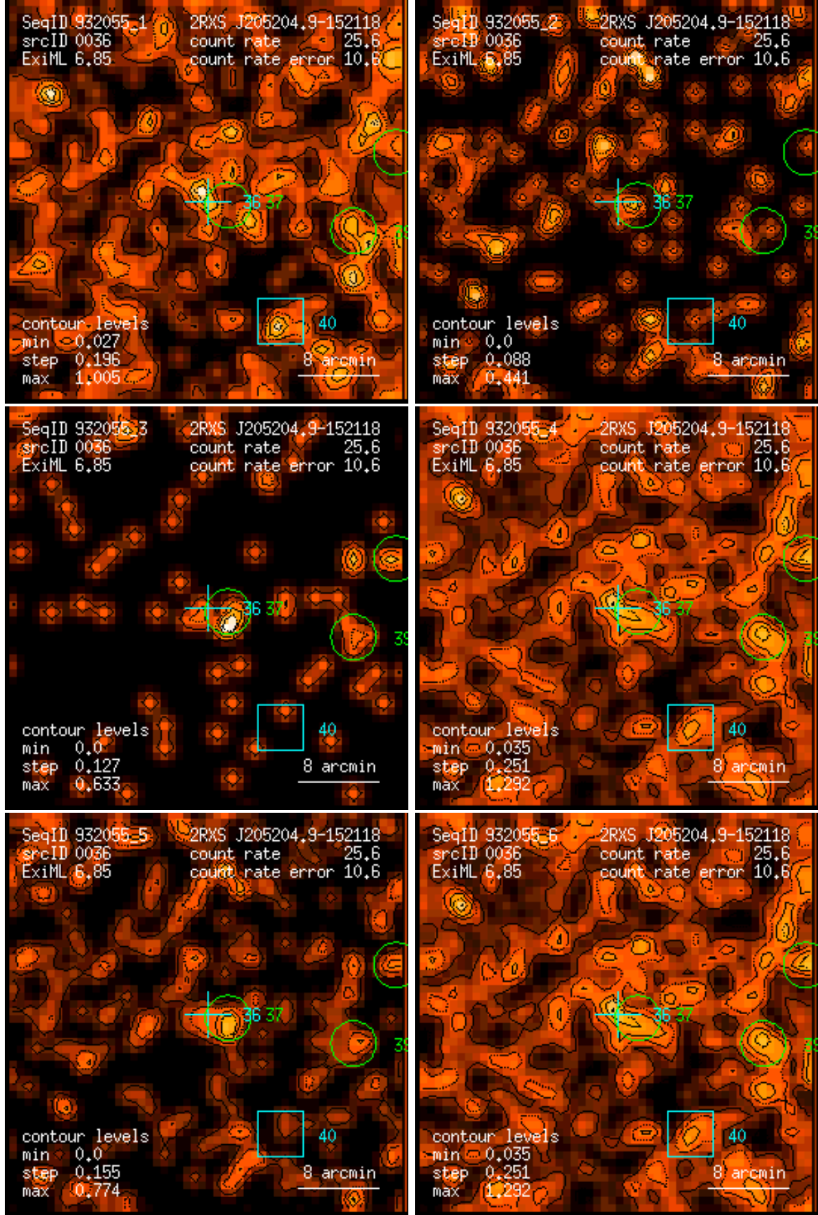
Figure 36: RASS 932055: detection 0036: band rate images, Gaussian filter: (1) PSPC channels 11 – 41, (2) 52 – 90, (3) 91 – 201, (4) 11 – 235, (5) 52 – 201, (6) 11 – 201. Broad band rates in counts/ks. Band rate contour levels in counts/ks/arcmin 2 .
