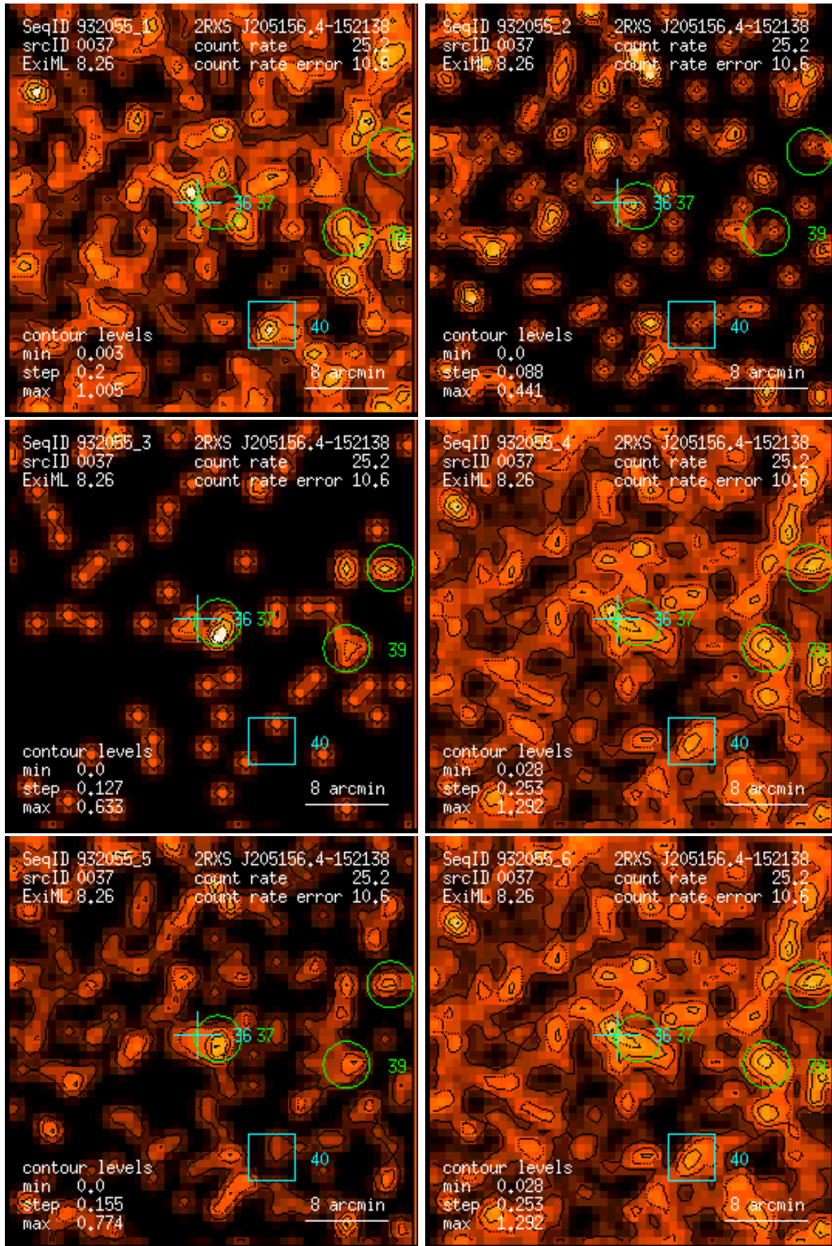
Figure 37: RASS 932055: detection 0037: band rate images, Gaussian filter: (1) PSPC channels 11 – 41, (2) 52 – 90, (3) 91 – 201, (4) 11 – 235, (5) 52 – 201, (6) 11 – 201. Broad band rates in counts/ks. Band rate contour levels in counts/ks/arcmin 2 .
