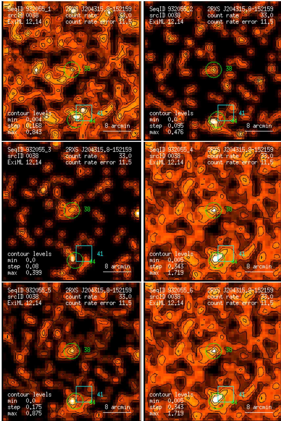
Figure 38: RASS 932055: detection 0038: band rate images, Gaussian filter: (1) PSPC channels 11 – 41, (2) 52 – 90, (3) 91 – 201, (4) 11 – 235, (5) 52 – 201, (6) 11 – 201. Broad band rates in counts/ks. Band rate contour levels in counts/ks/arcmin 2 .
