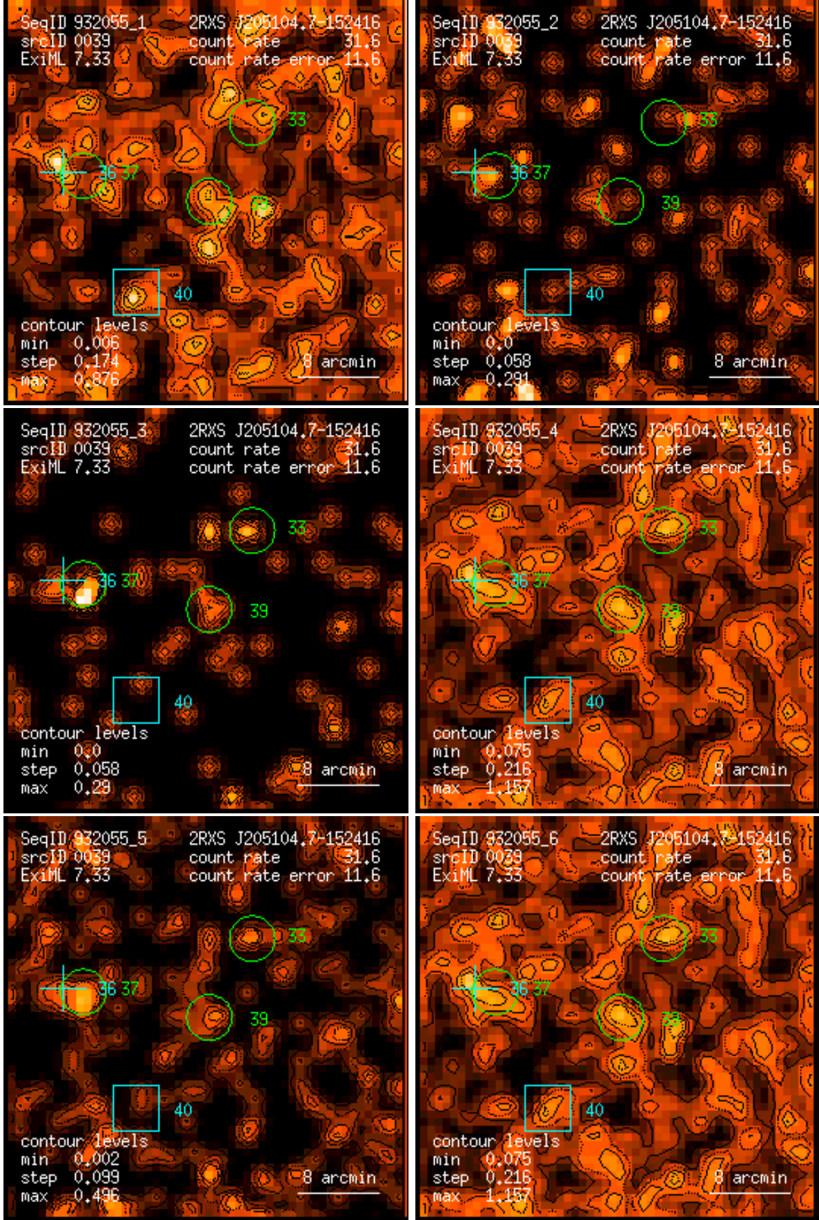
Figure 39: RASS 932055: detection 0039: band rate images, Gaussian filter: (1) PSPC channels 11 – 41, (2) 52 – 90, (3) 91 – 201, (4) 11 – 235, (5) 52 – 201, (6) 11 – 201. Broad band rates in counts/ks. Band rate contour levels in counts/ks/arcmin 2 .
