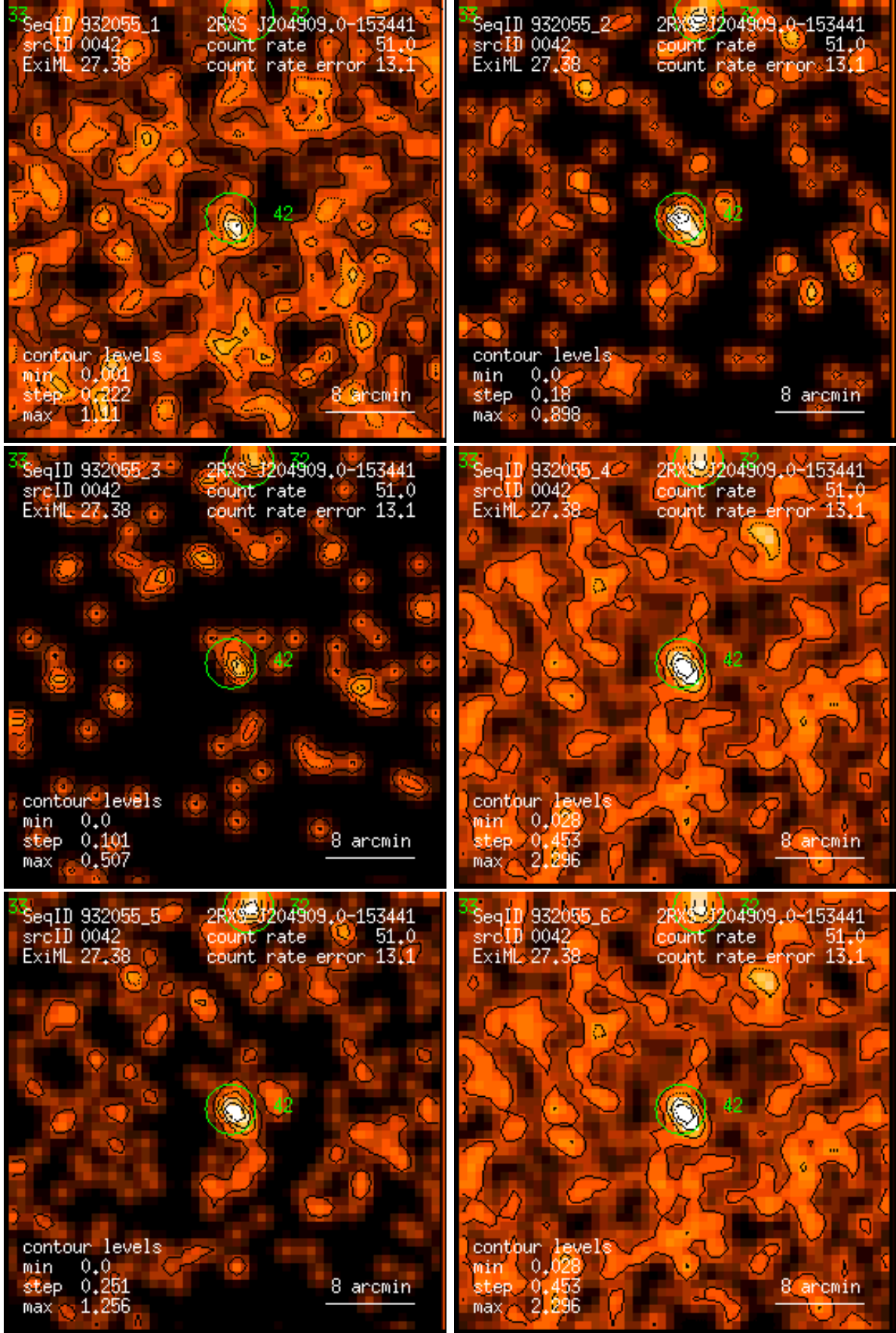
Figure 42: RASS 932055: detection 0042: band rate images, Gaussian filter: (1) PSPC channels 11 – 41, (2) 52 – 90, (3) 91 – 201, (4) 11 – 235, (5) 52 – 201, (6) 11 – 201. Broad band rates in counts/ks. Band rate contour levels in counts/ks/arcmin 2 .
