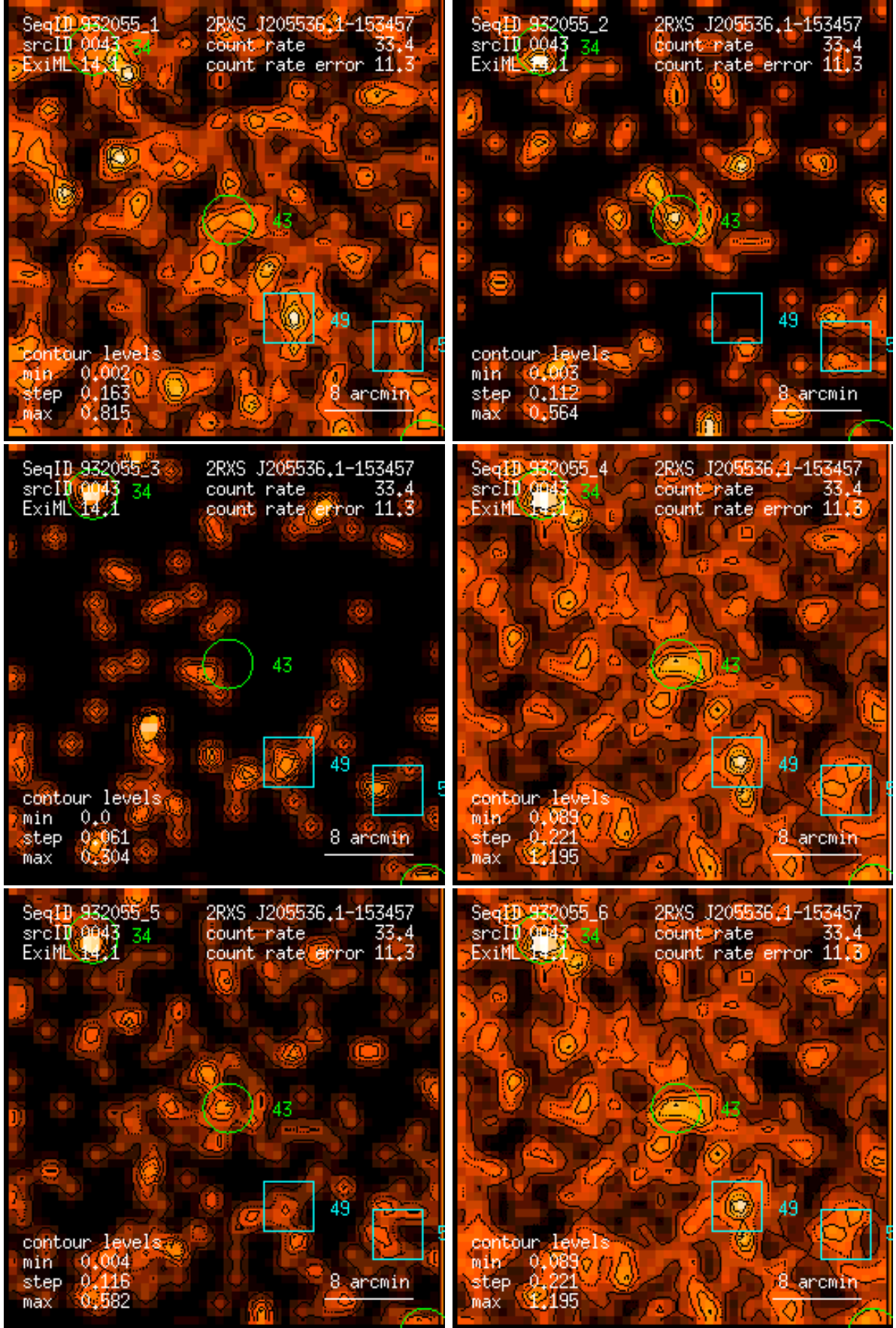
Figure 43: RASS 932055: detection 0043: band rate images, Gaussian filter: (1) PSPC channels 11 – 41, (2) 52 – 90, (3) 91 – 201, (4) 11 – 235, (5) 52 – 201, (6) 11 – 201. Broad band rates in counts/ks. Band rate contour levels in counts/ks/arcmin 2 .
