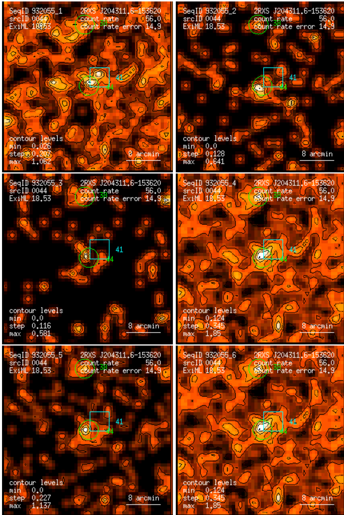
Figure 44: RASS 932055: detection 0044: band rate images, Gaussian filter: (1) PSPC channels 11 – 41, (2) 52 – 90, (3) 91 – 201, (4) 11 – 235, (5) 52 – 201, (6) 11 – 201. Broad band rates in counts/ks. Band rate contour levels in counts/ks/arcmin 2 .
