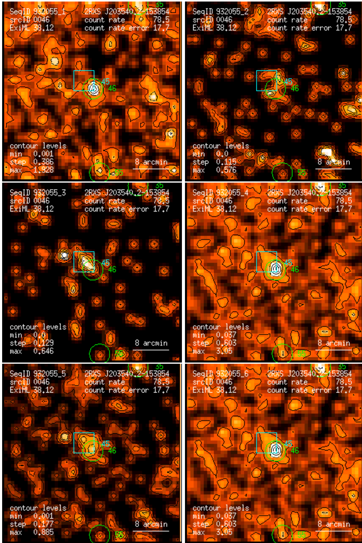
Figure 46: RASS 932055: detection 0046: band rate images, Gaussian filter: (1) PSPC channels 11 – 41, (2) 52 – 90, (3) 91 – 201, (4) 11 – 235, (5) 52 – 201, (6) 11 – 201. Broad band rates in counts/ks. Band rate contour levels in counts/ks/arcmin 2 .
