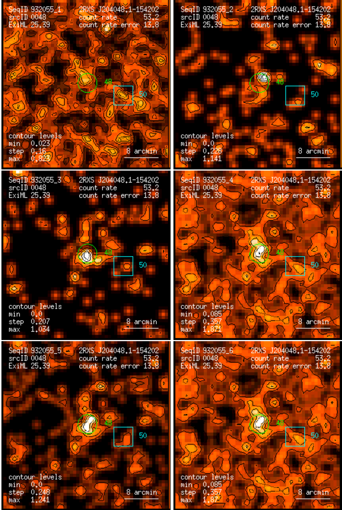
Figure 48: RASS 932055: detection 0048: band rate images, Gaussian filter: (1) PSPC channels 11 – 41, (2) 52 – 90, (3) 91 – 201, (4) 11 – 235, (5) 52 – 201, (6) 11 – 201. Broad band rates in counts/ks. Band rate contour levels in counts/ks/arcmin 2 .
