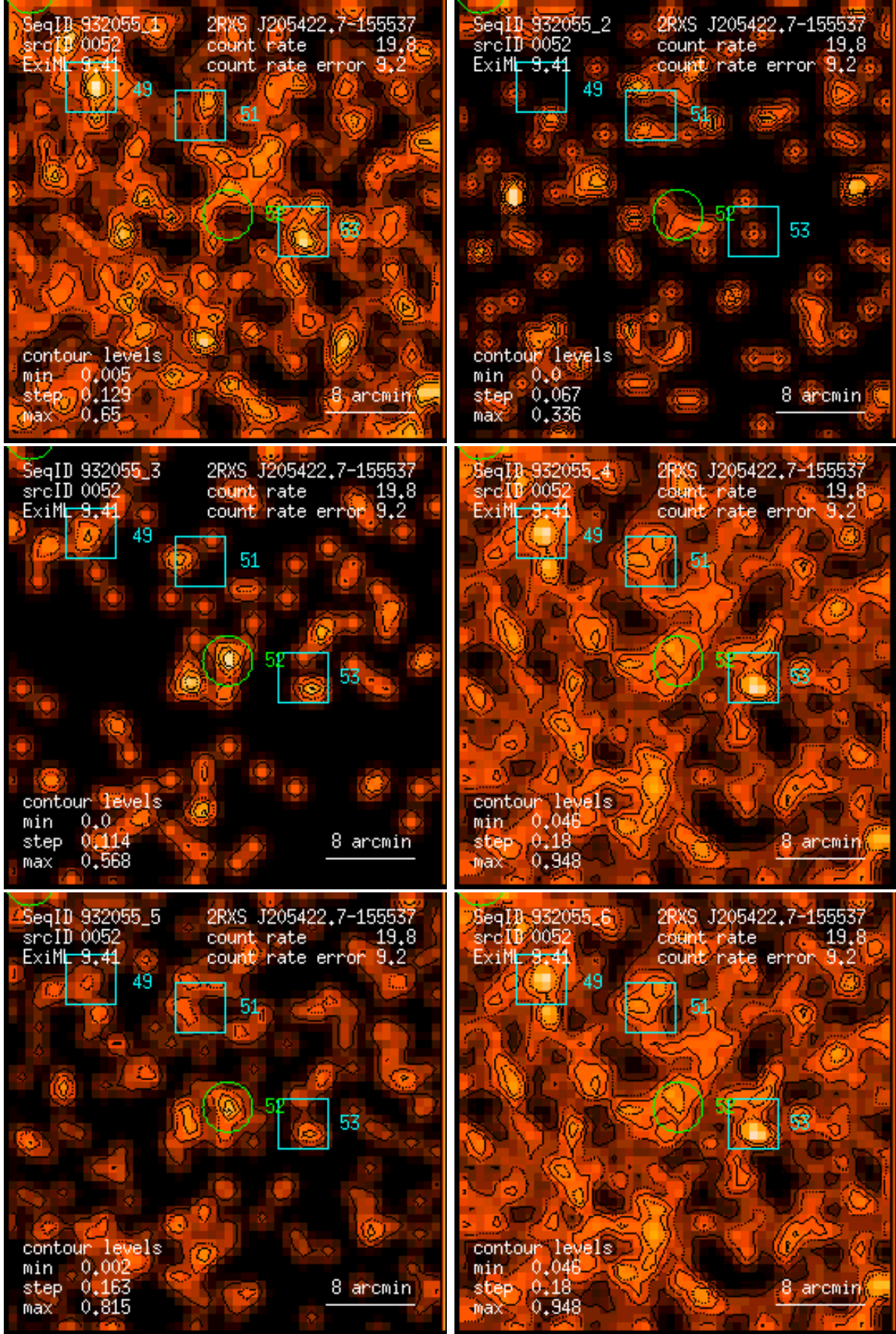
Figure 52: RASS 932055: detection 0052: band rate images, Gaussian filter: (1) PSPC channels 11 – 41, (2) 52 – 90, (3) 91 – 201, (4) 11 – 235, (5) 52 – 201, (6) 11 – 201. Broad band rates in counts/ks. Band rate contour levels in counts/ks/arcmin 2 .
