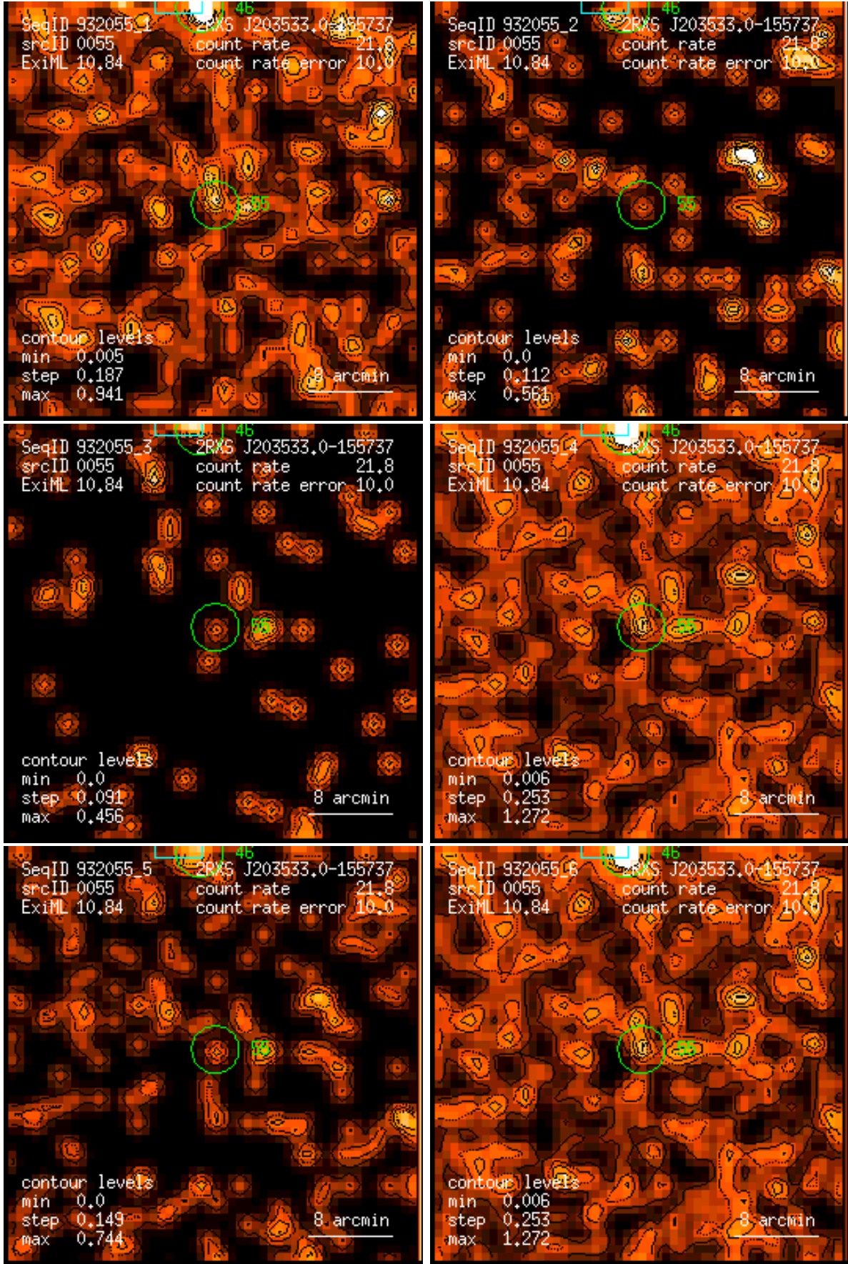
Figure 55: RASS 932055: detection 0055: band rate images, Gaussian filter: (1) PSPC channels 11 – 41, (2) 52 – 90, (3) 91 – 201, (4) 11 – 235, (5) 52 – 201, (6) 11 – 201. Broad band rates in counts/ks. Band rate contour levels in counts/ks/arcmin 2 .
