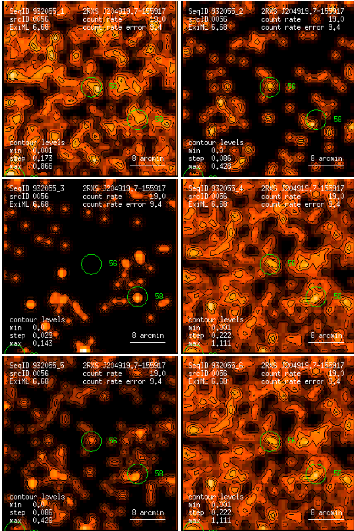
Figure 56: RASS 932055: detection 0056: band rate images, Gaussian filter: (1) PSPC channels 11 – 41, (2) 52 – 90, (3) 91 – 201, (4) 11 – 235, (5) 52 – 201, (6) 11 – 201. Broad band rates in counts/ks. Band rate contour levels in counts/ks/arcmin 2 .
