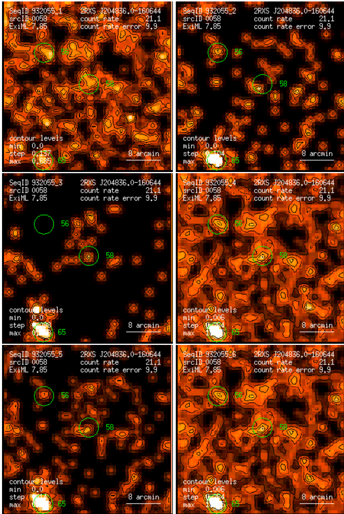
Figure 58: RASS 932055: detection 0058: band rate images, Gaussian filter: (1) PSPC channels 11 – 41, (2) 52 – 90, (3) 91 – 201, (4) 11 – 235, (5) 52 – 201, (6) 11 – 201. Broad band rates in counts/ks. Band rate contour levels in counts/ks/arcmin 2 .
