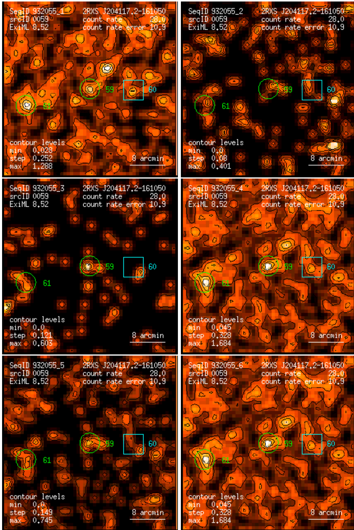
Figure 59: RASS 932055: detection 0059: band rate images, Gaussian filter: (1) PSPC channels 11 – 41, (2) 52 – 90, (3) 91 – 201, (4) 11 – 235, (5) 52 – 201, (6) 11 – 201. Broad band rates in counts/ks. Band rate contour levels in counts/ks/arcmin 2 .
