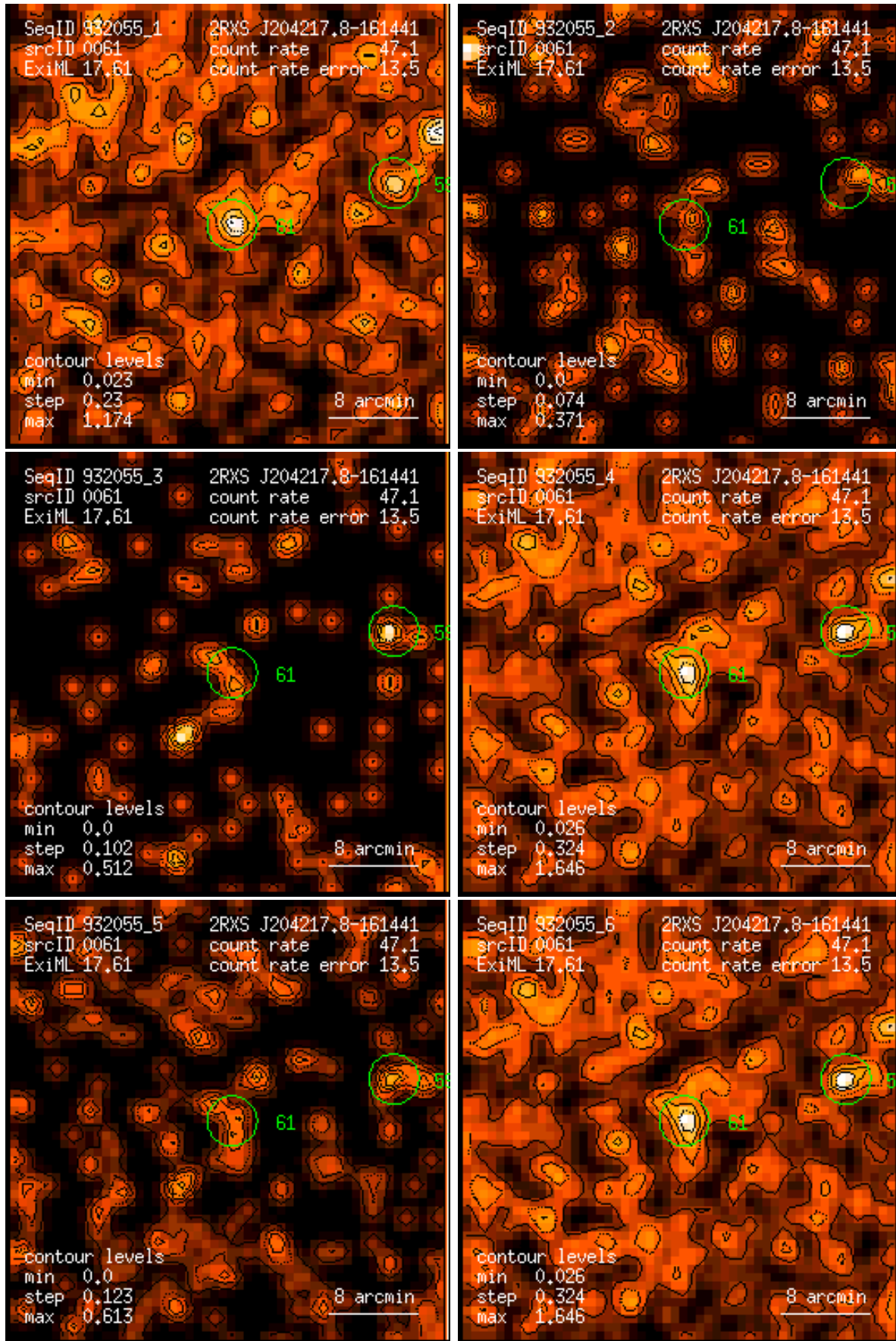
Figure 61: RASS 932055: detection 0061: band rate images, Gaussian filter: (1) PSPC channels 11 – 41, (2) 52 – 90, (3) 91 – 201, (4) 11 – 235, (5) 52 – 201, (6) 11 – 201. Broad band rates in counts/ks. Band rate contour levels in counts/ks/arcmin 2 .
