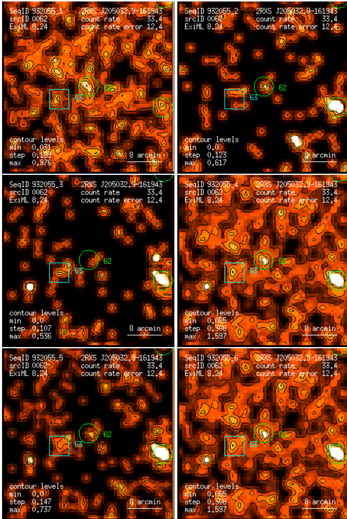
Figure 62: RASS 932055: detection 0062: band rate images, Gaussian filter: (1) PSPC channels 11 – 41, (2) 52 – 90, (3) 91 – 201, (4) 11 – 235, (5) 52 – 201, (6) 11 – 201. Broad band rates in counts/ks. Band rate contour levels in counts/ks/arcmin 2 .
