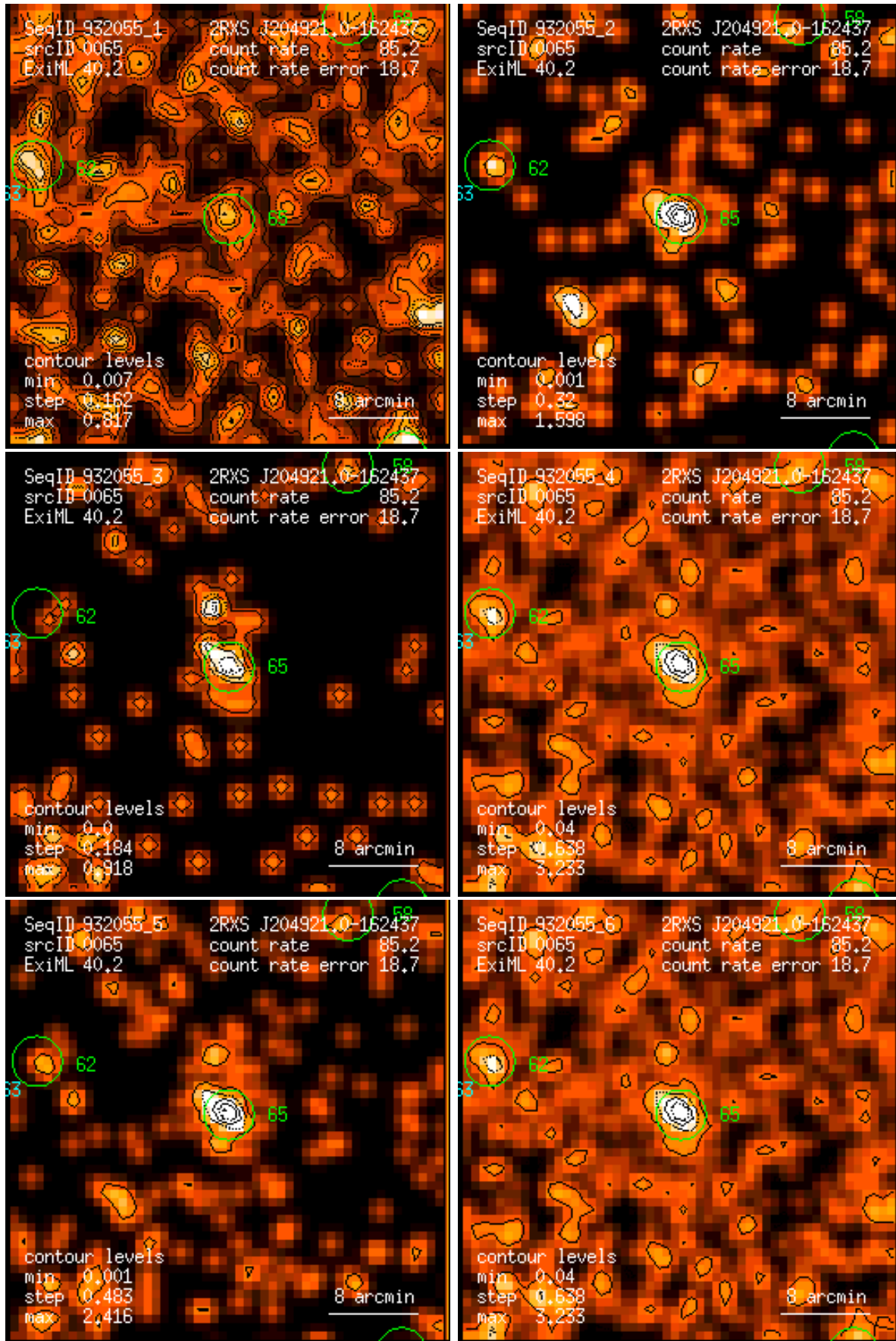
Figure 65: RASS 932055: detection 0065: band rate images, Gaussian filter: (1) PSPC channels 11 – 41, (2) 52 – 90, (3) 91 – 201, (4) 11 – 235, (5) 52 – 201, (6) 11 – 201. Broad band rates in counts/ks. Band rate contour levels in counts/ks/arcmin 2 .
