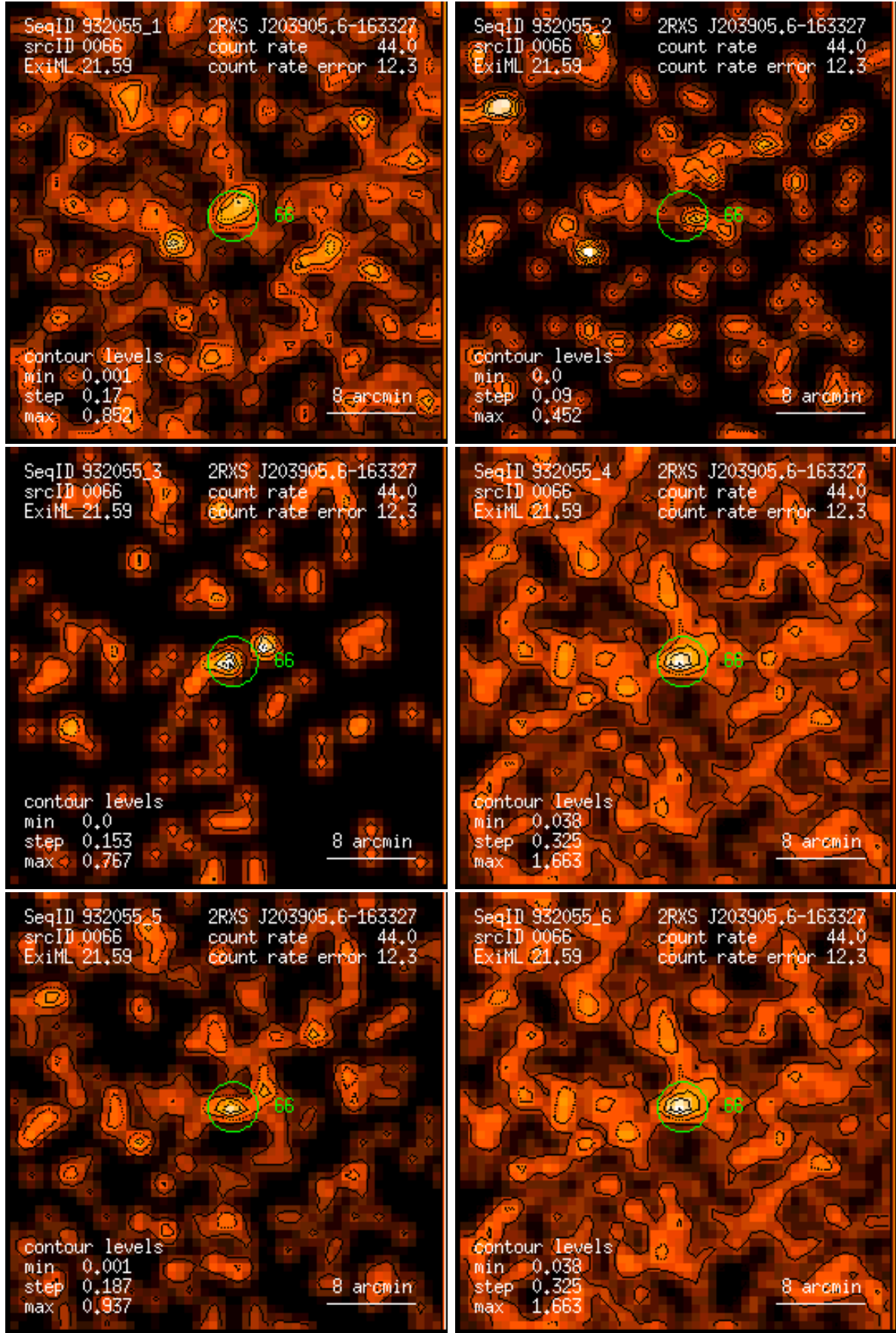
Figure 66: RASS 932055: detection 0066: band rate images, Gaussian filter: (1) PSPC channels 11 – 41, (2) 52 – 90, (3) 91 – 201, (4) 11 – 235, (5) 52 – 201, (6) 11 – 201. Broad band rates in counts/ks. Band rate contour levels in counts/ks/arcmin 2 .
