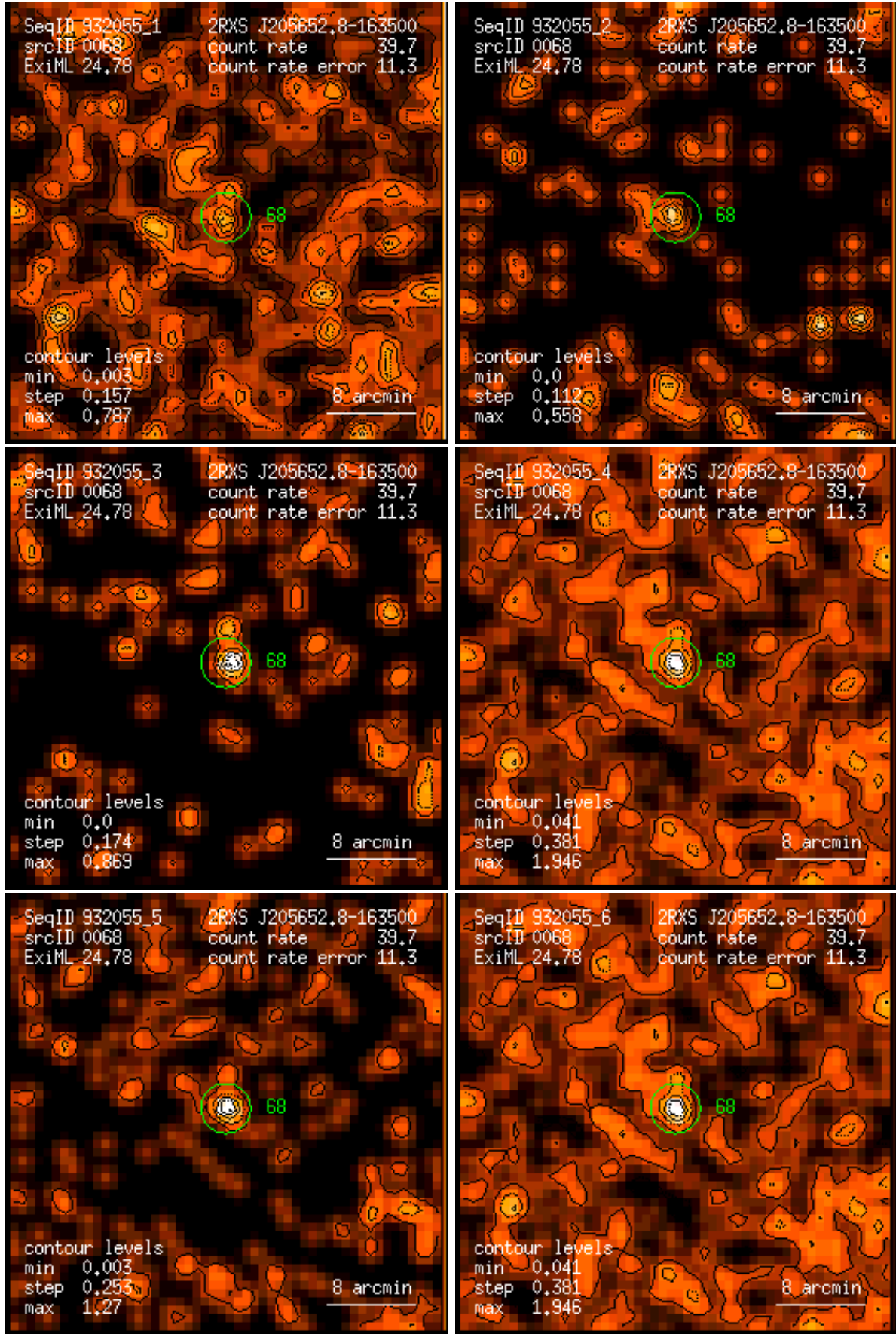
Figure 68: RASS 932055: detection 0068: band rate images, Gaussian filter: (1) PSPC channels 11 – 41, (2) 52 – 90, (3) 91 – 201, (4) 11 – 235, (5) 52 – 201, (6) 11 – 201. Broad band rates in counts/ks. Band rate contour levels in counts/ks/arcmin 2 .
