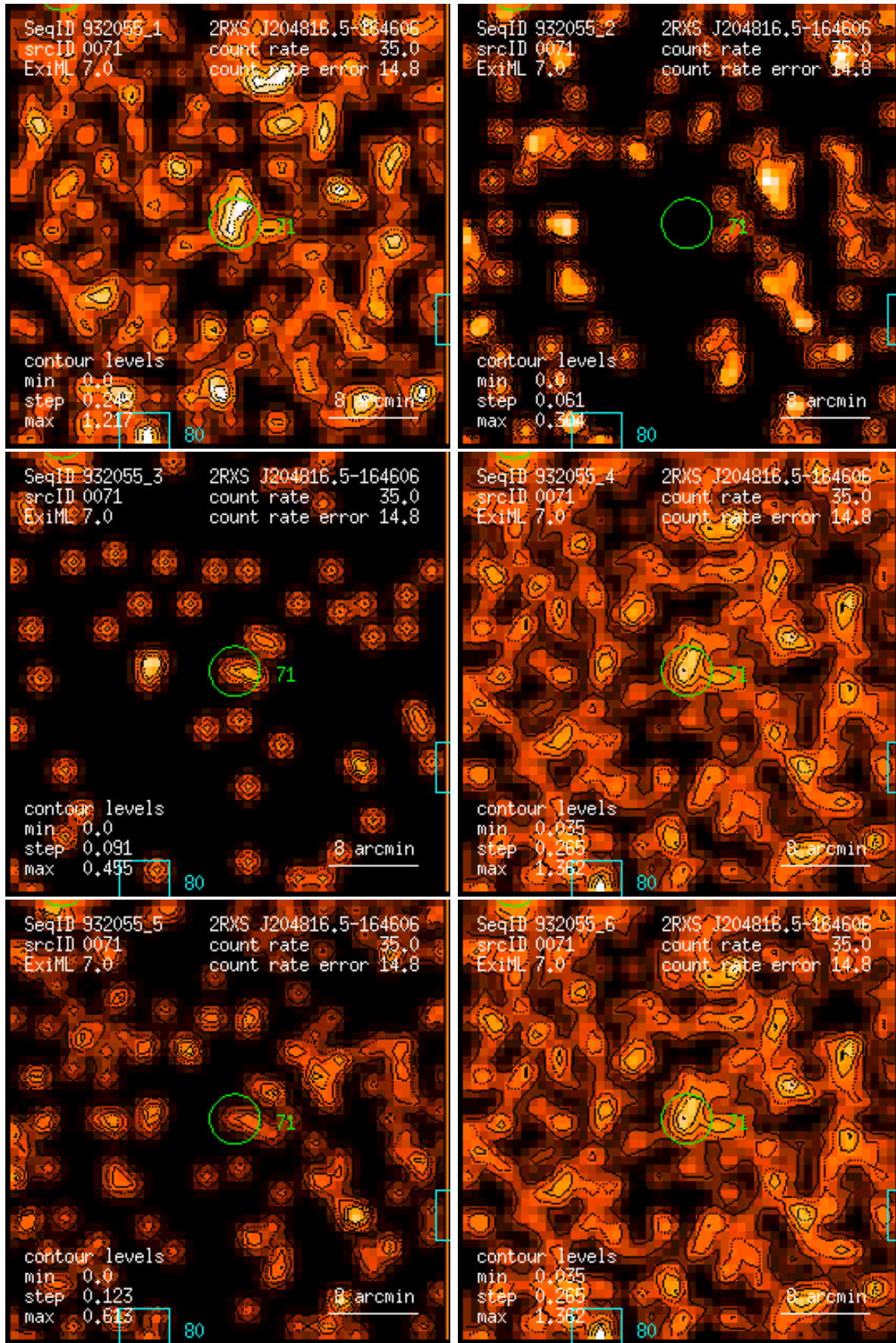
Figure 71: RASS 932055: detection 0071: band rate images, Gaussian filter: (1) PSPC channels 11 – 41, (2) 52 – 90, (3) 91 – 201, (4) 11 – 235, (5) 52 – 201, (6) 11 – 201. Broad band rates in counts/ks. Band rate contour levels in counts/ks/arcmin 2 .
