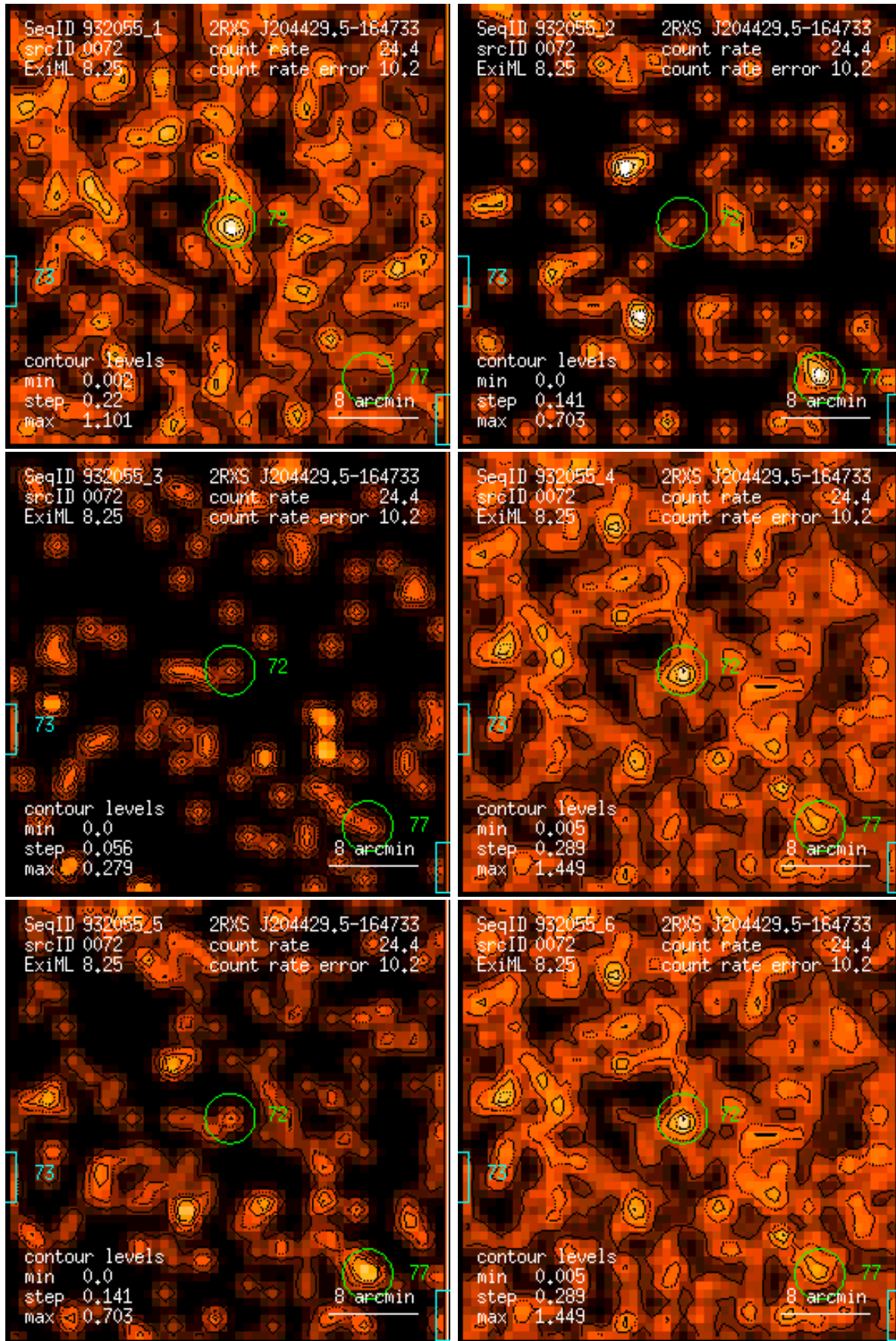
Figure 72: RASS 932055: detection 0072: band rate images, Gaussian filter: (1) PSPC channels 11 – 41, (2) 52 – 90, (3) 91 – 201, (4) 11 – 235, (5) 52 – 201, (6) 11 – 201. Broad band rates in counts/ks. Band rate contour levels in counts/ks/arcmin 2 .
