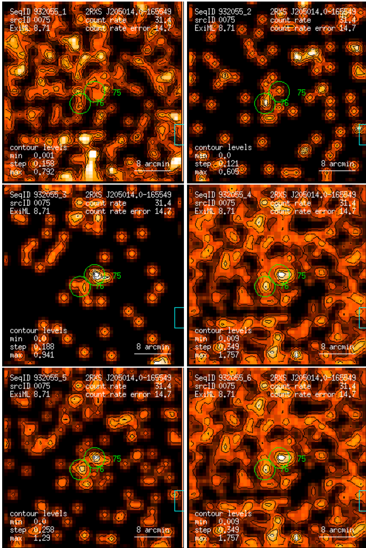
Figure 75: RASS 932055: detection 0075: band rate images, Gaussian filter: (1) PSPC channels 11 – 41, (2) 52 – 90, (3) 91 – 201, (4) 11 – 235, (5) 52 – 201, (6) 11 – 201. Broad band rates in counts/ks. Band rate contour levels in counts/ks/arcmin 2 .
