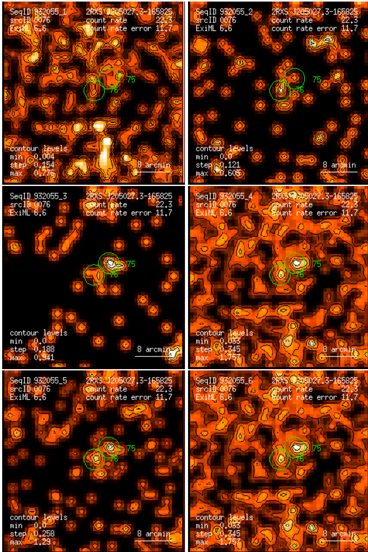
Figure 76: RASS 932055: detection 0076: band rate images, Gaussian filter: (1) PSPC channels 11 – 41, (2) 52 – 90, (3) 91 – 201, (4) 11 – 235, (5) 52 – 201, (6) 11 – 201. Broad band rates in counts/ks. Band rate contour levels in counts/ks/arcmin 2 .
