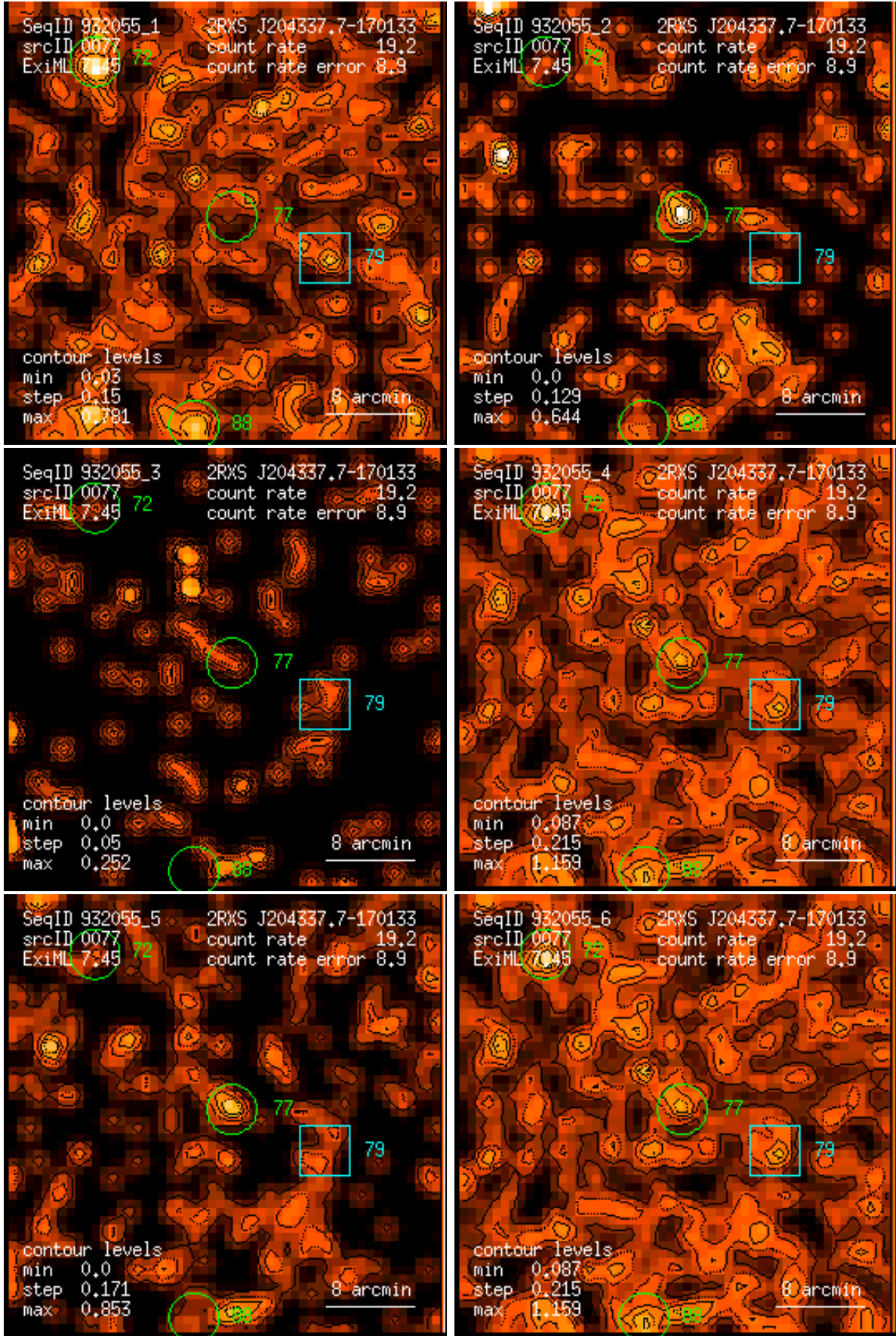
Figure 77: RASS 932055: detection 0077: band rate images, Gaussian filter: (1) PSPC channels 11 – 41, (2) 52 – 90, (3) 91 – 201, (4) 11 – 235, (5) 52 – 201, (6) 11 – 201. Broad band rates in counts/ks. Band rate contour levels in counts/ks/arcmin 2 .
