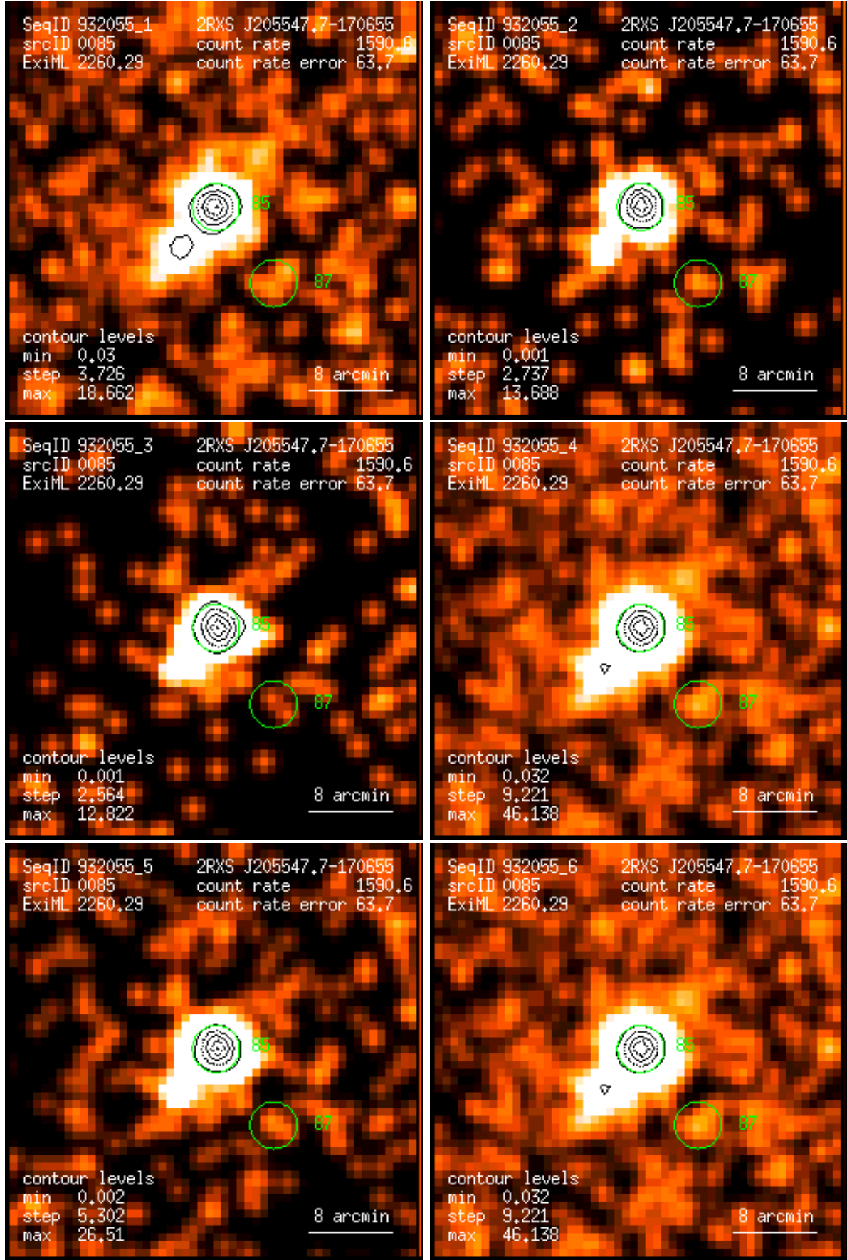
Figure 85: RASS 932055: detection 0085: band rate images, Gaussian filter: (1) PSPC channels 11 – 41, (2) 52 – 90, (3) 91 – 201, (4) 11 – 235, (5) 52 – 201, (6) 11 – 201. Broad band rates in counts/ks. Band rate contour levels in counts/ks/arcmin 2 .
