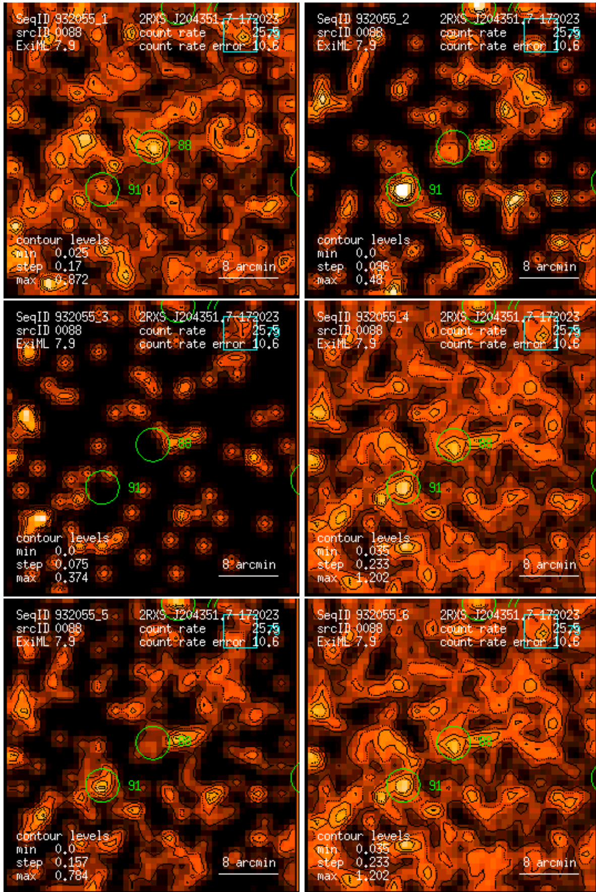
Figure 88: RASS 932055: detection 0088: band rate images, Gaussian filter: (1) PSPC channels 11 – 41, (2) 52 – 90, (3) 91 – 201, (4) 11 – 235, (5) 52 – 201, (6) 11 – 201. Broad band rates in counts/ks. Band rate contour levels in counts/ks/arcmin 2 .
