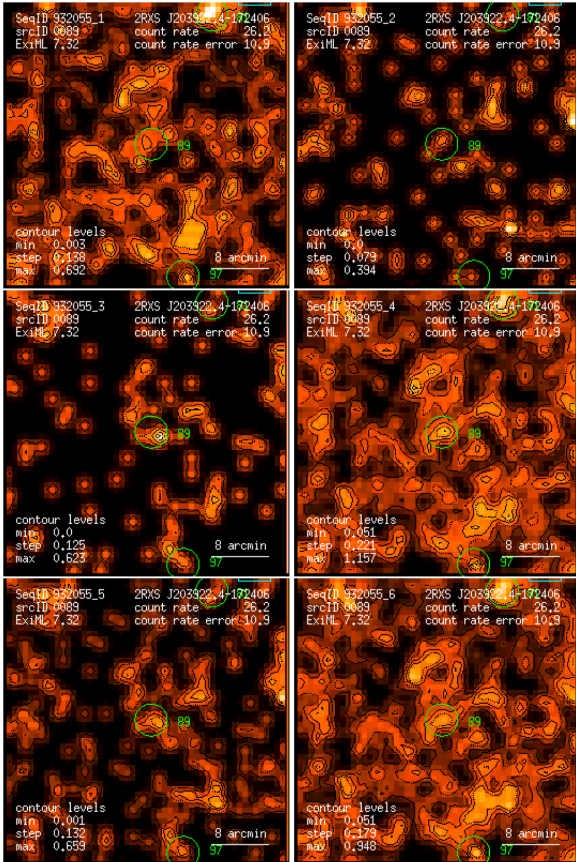
Figure 89: RASS 932055: detection 0089: band rate images, Gaussian filter: (1) PSPC channels 11 – 41, (2) 52 – 90, (3) 91 – 201, (4) 11 – 235, (5) 52 – 201, (6) 11 – 201. Broad band rates in counts/ks. Band rate contour levels in counts/ks/arcmin 2 .
