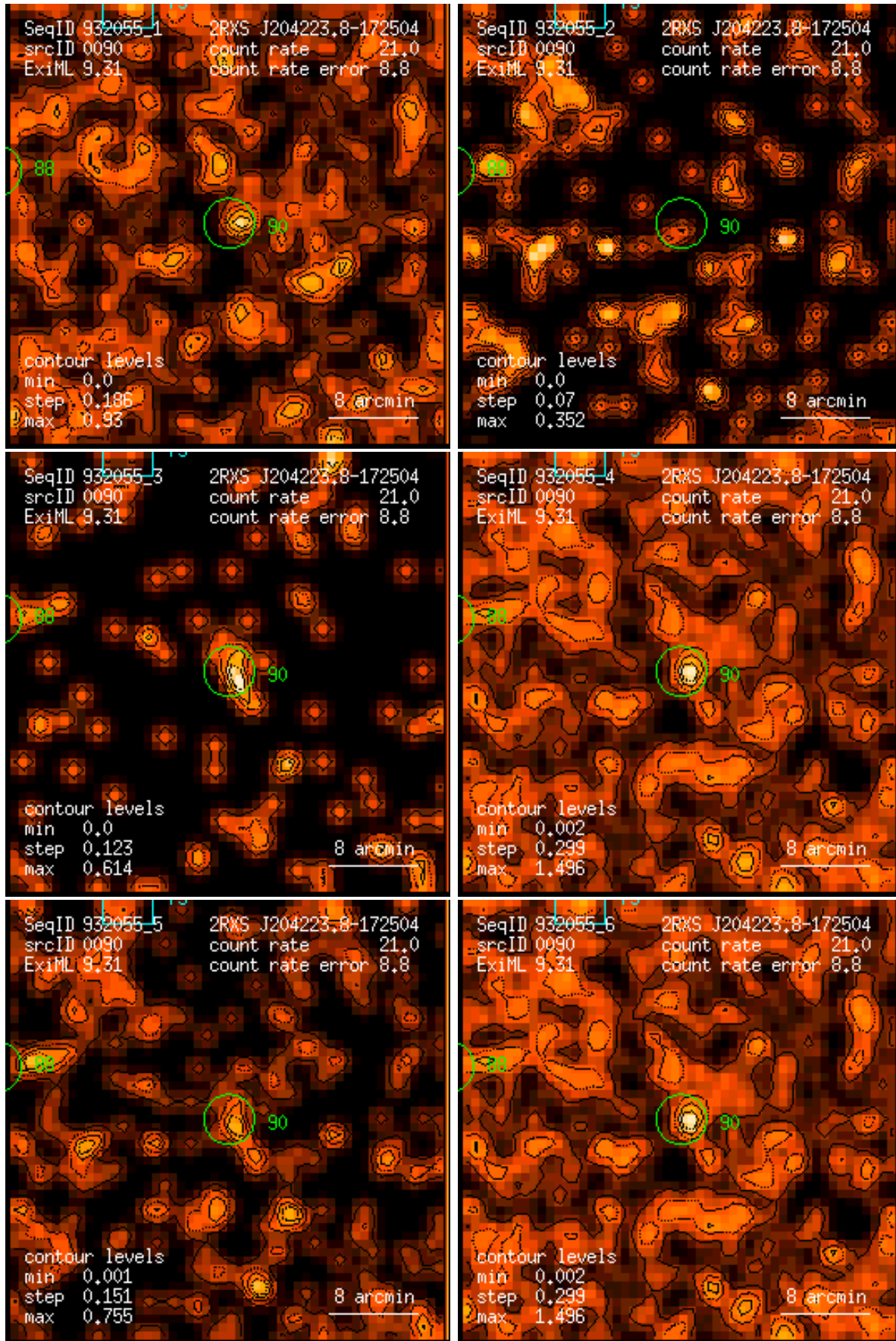
Figure 90: RASS 932055: detection 0090: band rate images, Gaussian filter: (1) PSPC channels 11 – 41, (2) 52 – 90, (3) 91 – 201, (4) 11 – 235, (5) 52 – 201, (6) 11 – 201. Broad band rates in counts/ks. Band rate contour levels in counts/ks/arcmin 2 .
