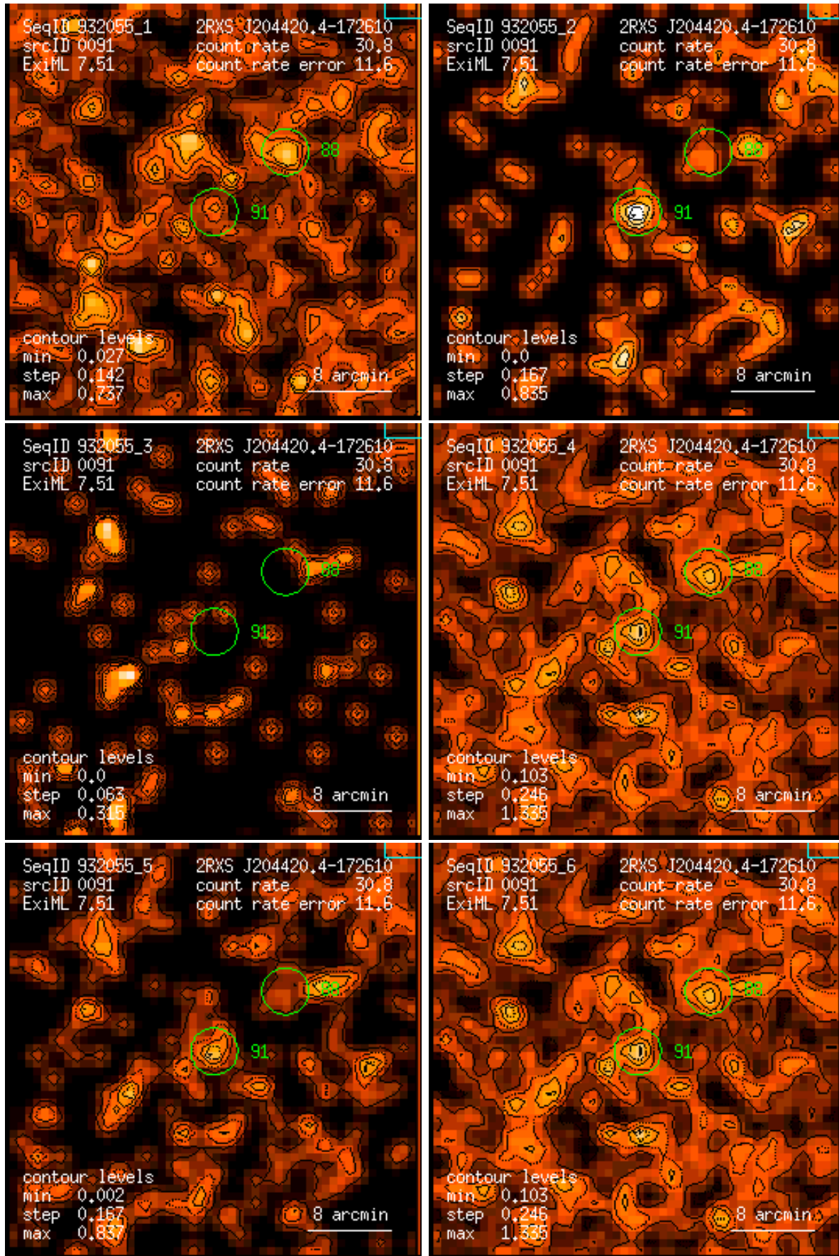
Figure 91: RASS 932055: detection 0091: band rate images, Gaussian filter: (1) PSPC channels 11 – 41, (2) 52 – 90, (3) 91 – 201, (4) 11 – 235, (5) 52 – 201, (6) 11 – 201. Broad band rates in counts/ks. Band rate contour levels in counts/ks/arcmin 2 .
