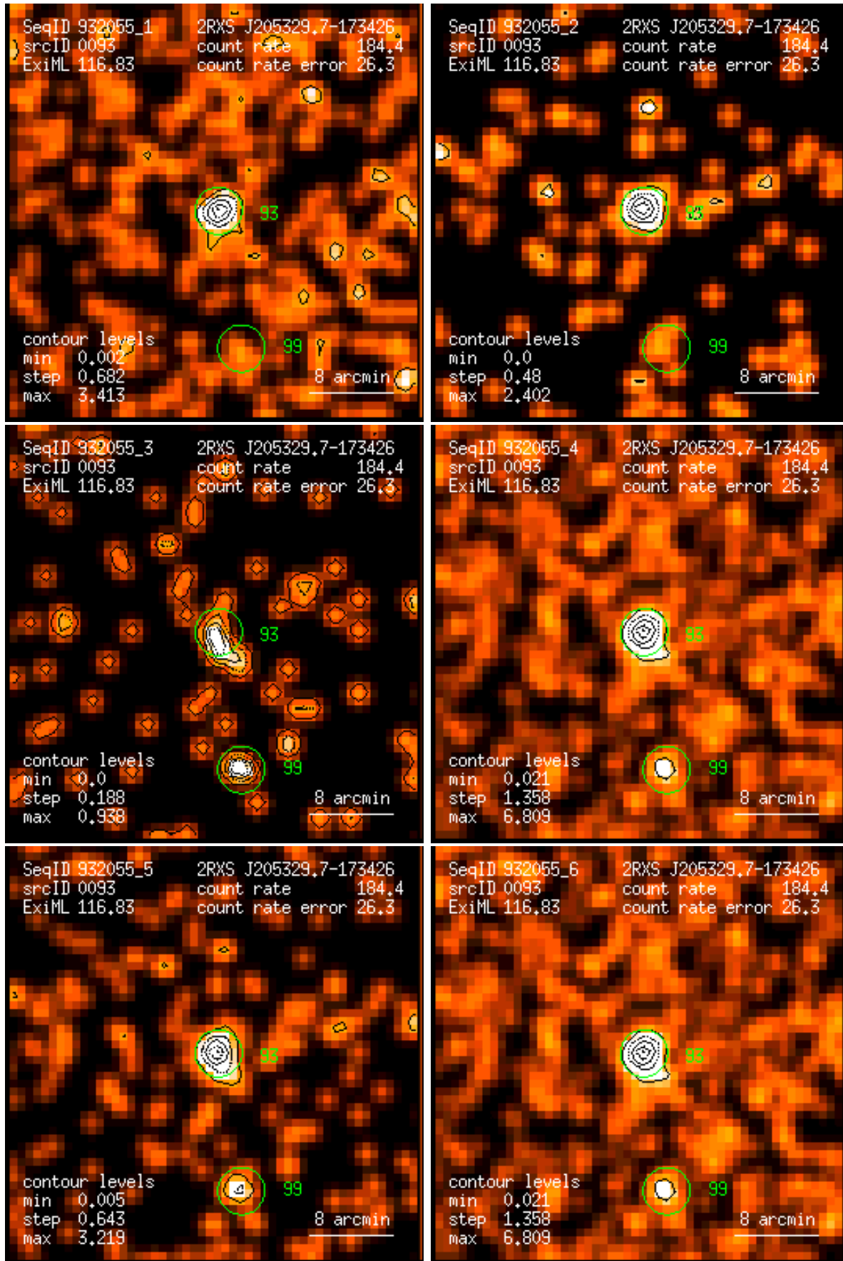
Figure 93: RASS 932055: detection 0093: band rate images, Gaussian filter: (1) PSPC channels 11 – 41, (2) 52 – 90, (3) 91 – 201, (4) 11 – 235, (5) 52 – 201, (6) 11 – 201. Broad band rates in counts/ks. Band rate contour levels in counts/ks/arcmin 2 .
