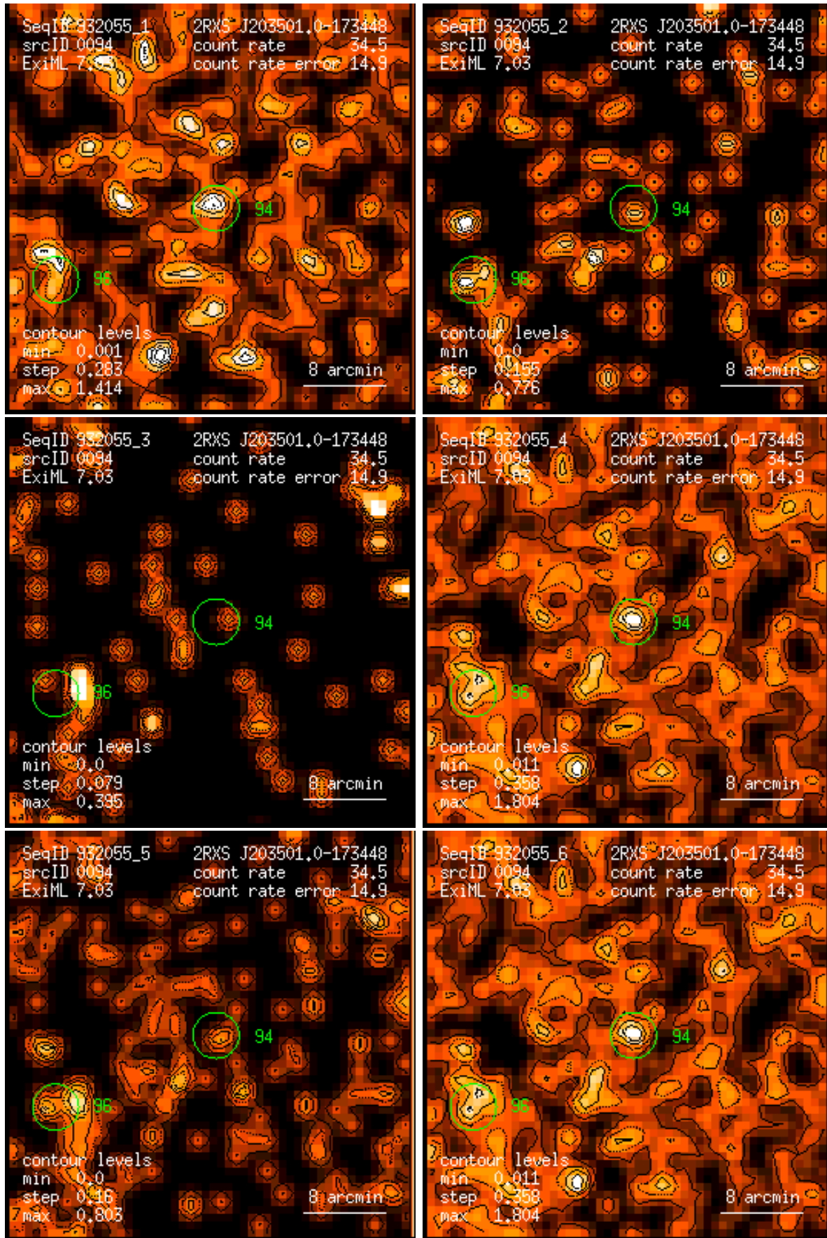
Figure 94: RASS 932055: detection 0094: band rate images, Gaussian filter: (1) PSPC channels 11 – 41, (2) 52 – 90, (3) 91 – 201, (4) 11 – 235, (5) 52 – 201, (6) 11 – 201. Broad band rates in counts/ks. Band rate contour levels in counts/ks/arcmin 2 .
