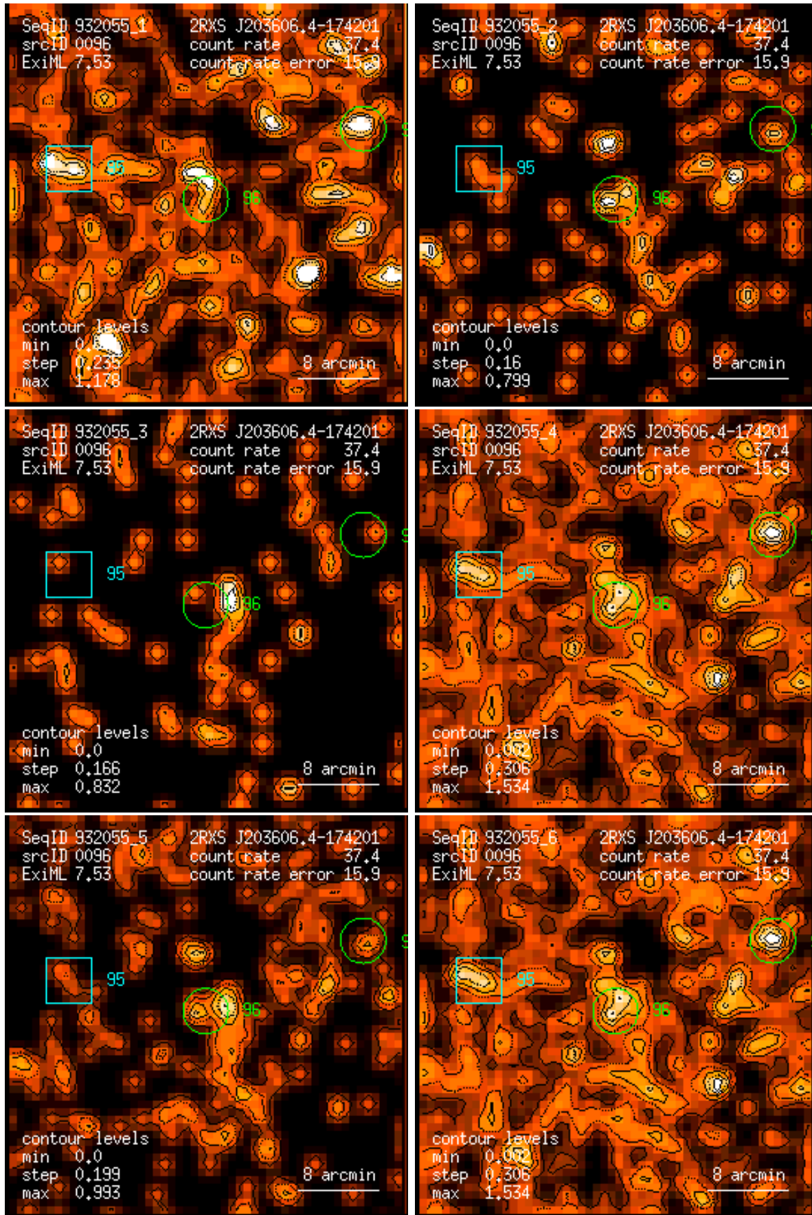
Figure 96: RASS 932055: detection 0096: band rate images, Gaussian filter: (1) PSPC channels 11 – 41, (2) 52 – 90, (3) 91 – 201, (4) 11 – 235, (5) 52 – 201, (6) 11 – 201. Broad band rates in counts/ks. Band rate contour levels in counts/ks/arcmin 2 .
