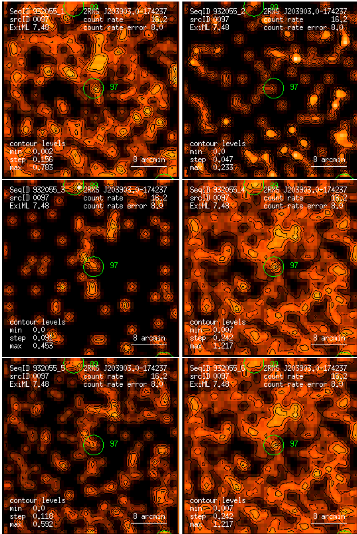
Figure 97: RASS 932055: detection 0097: band rate images, Gaussian filter: (1) PSPC channels 11 – 41, (2) 52 – 90, (3) 91 – 201, (4) 11 – 235, (5) 52 – 201, (6) 11 – 201. Broad band rates in counts/ks. Band rate contour levels in counts/ks/arcmin 2 .
