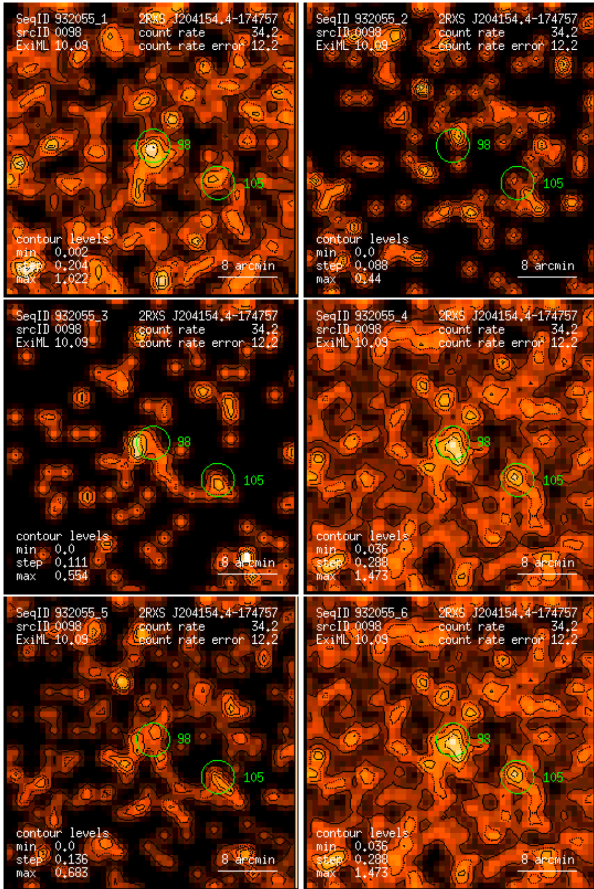
Figure 98: RASS 932055: detection 0098: band rate images, Gaussian filter: (1) PSPC channels 11 – 41, (2) 52 – 90, (3) 91 – 201, (4) 11 – 235, (5) 52 – 201, (6) 11 – 201. Broad band rates in counts/ks. Band rate contour levels in counts/ks/arcmin 2 .
