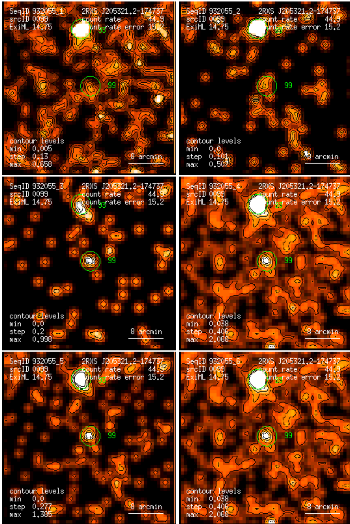
Figure 99: RASS 932055: detection 0099: band rate images, Gaussian filter: (1) PSPC channels 11 – 41, (2) 52 – 90, (3) 91 – 201, (4) 11 – 235, (5) 52 – 201, (6) 11 – 201. Broad band rates in counts/ks. Band rate contour levels in counts/ks/arcmin 2 .
