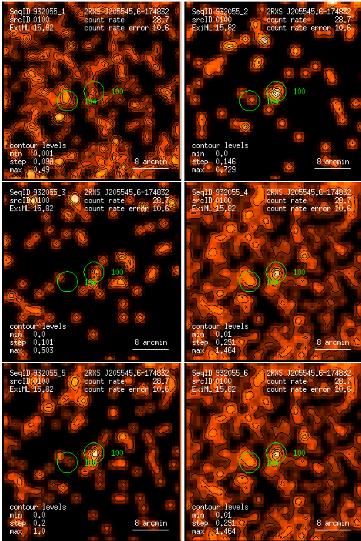
Figure 100: RASS 932055: detection 0100: band rate images, Gaussian filter: (1) PSPC channels 11 – 41, (2) 52 – 90, (3) 91 – 201, (4) 11 – 235, (5) 52 – 201, (6) 11 – 201. Broad band rates in counts/ks. Band rate contour levels in counts/ks/arcmin 2 .
